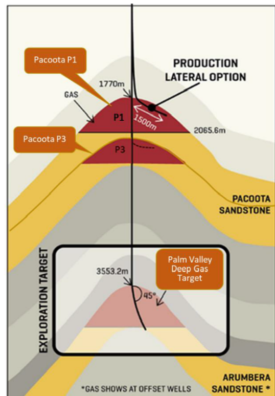
Figure 1. PV12 well schematic Source: New Zealand Oil & Gas
