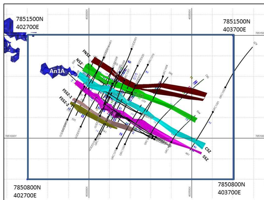
Figure 5 Plan view of the mineralized lenses at Goanna showing proximity to the Gecko Anomaly 1A mineralisation
