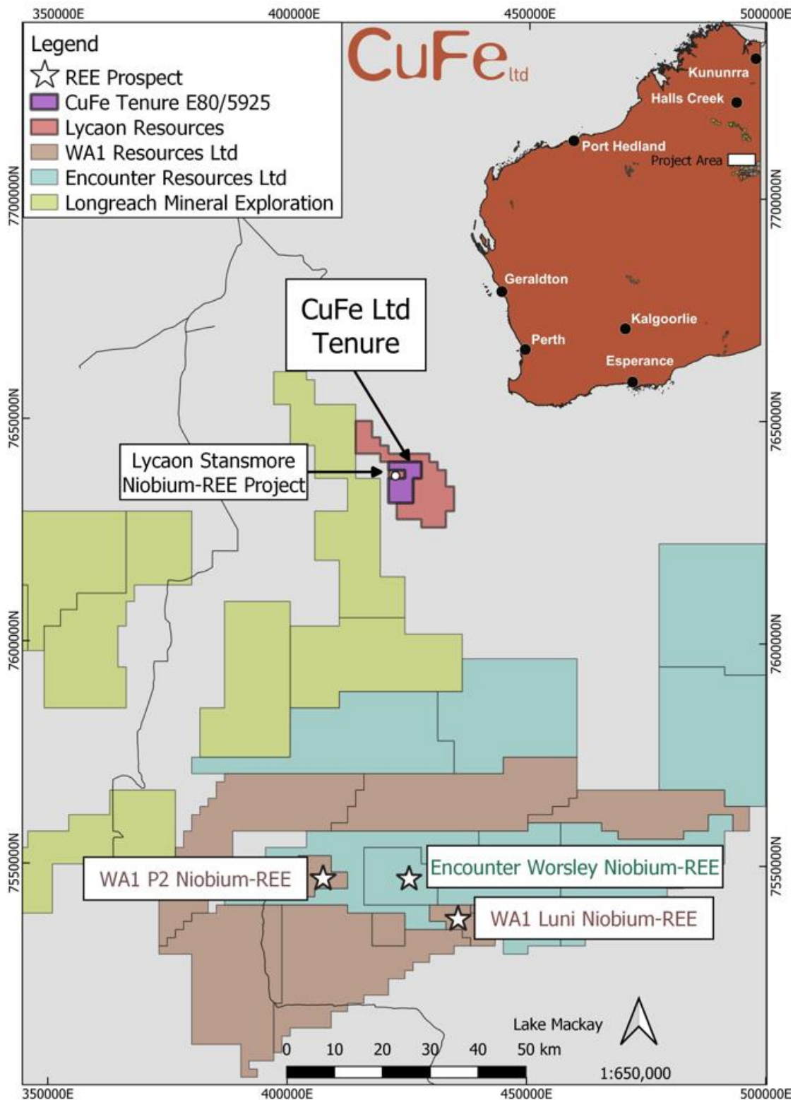
Figure 1: E80/5925 West Arunta location and proximity to neighbouring explorers.
