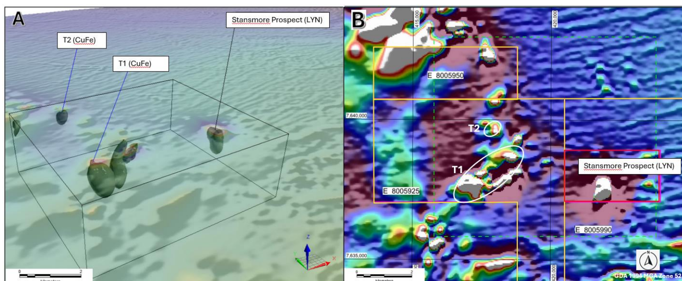
Figure 2: 3D inversion modelling of the T1 and T2 magnetic anomalies.
