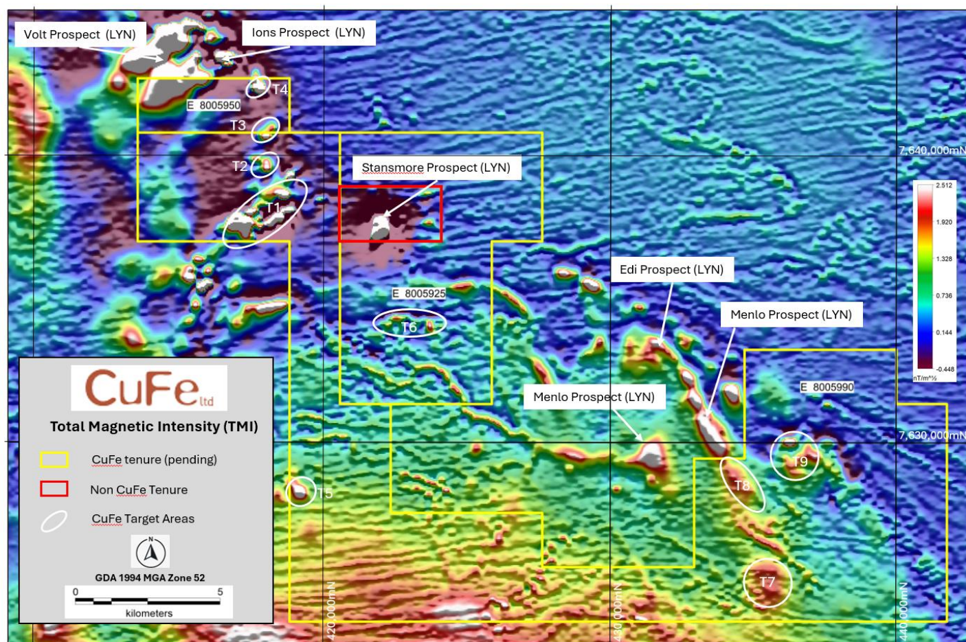
Figure 1: Total Magnetic Intensity (TMI) and location of Target areas T1 to T9.
