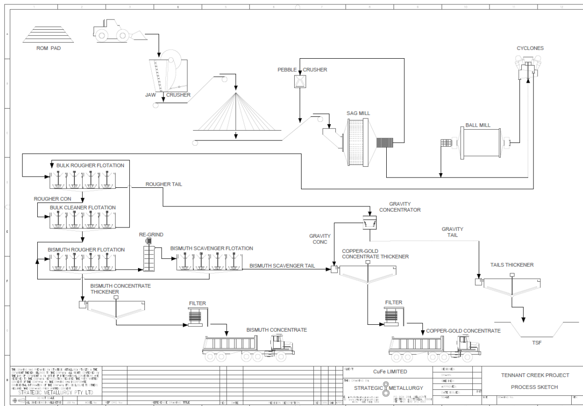
Figure 10: Process Block flow diagram
