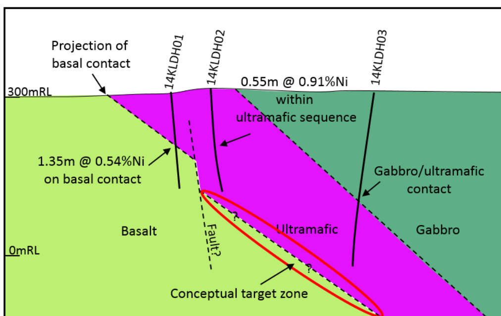
Figure 2: Killaloe HWG conceptual geological target
