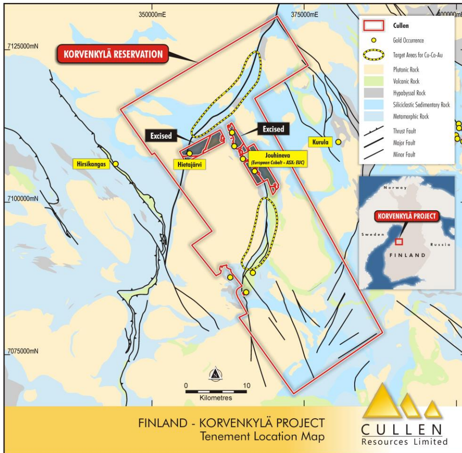
Fig. 6 : Jousineva prospect (European Cobalt) includes reported intersections of : 5.55m @ 1.19% Co in drillhole KJ-JO-057 from 23m; including: 0.45m at 5.63% Co, 4.7g/t Au from 23m and 0.70m at 4.04% Co from 24.65m: ( www.europeancobalt.com ).
