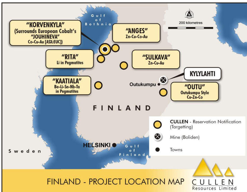
Fig. 6 : Jousineva prospect (European Cobalt) includes reported intersections of : 5.55m @ 1.19% Co in drillhole KJ-JO-057 from 23m; including: 0.45m at 5.63% Co, 4.7g/t Au from 23m and 0.70m at 4.04% Co from 24.65m: ( www.europeancobalt.com ).
