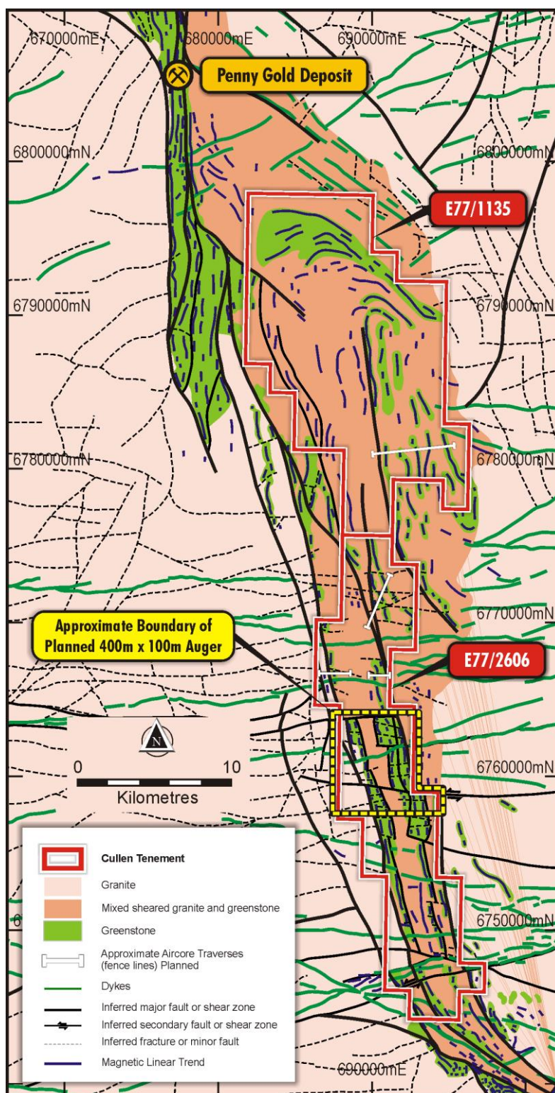
Fig.9 Interpretation of air magnetic data, south east of the Youanmi greenstone belt – air core traverses and auger sampling planned.
