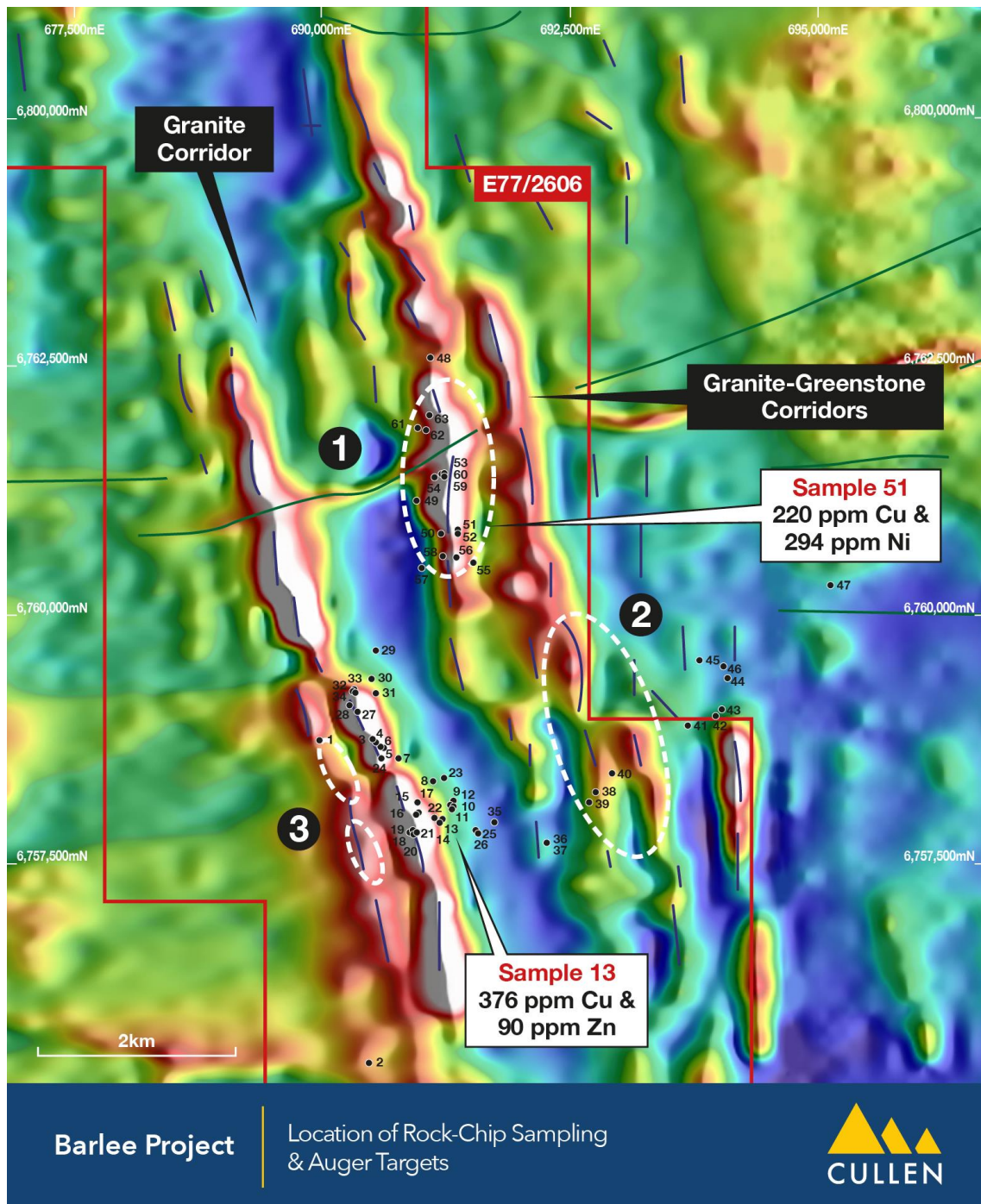
Fig.14 Magnetics image
