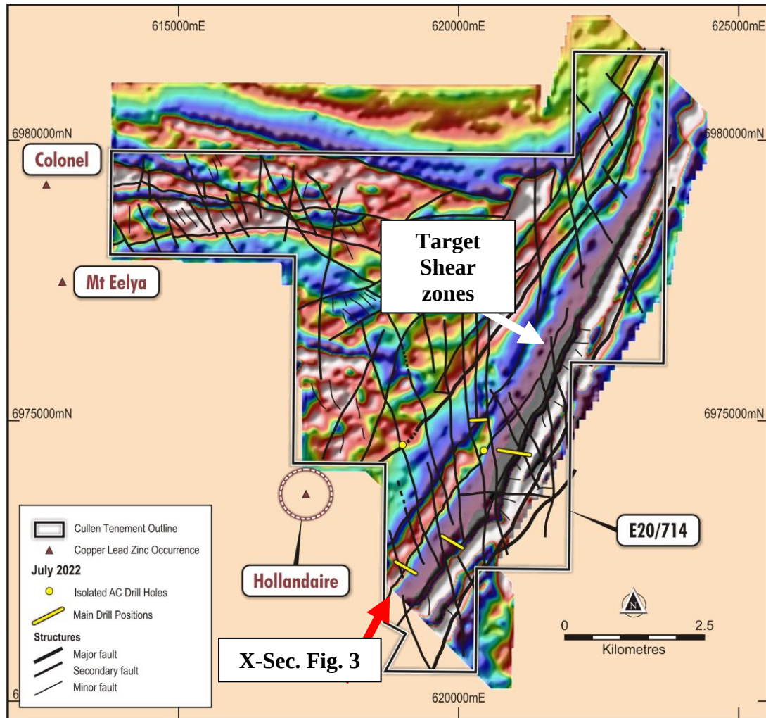
Fig. 2. Key structural lineaments overlain on magnetic image Image (TMI) from Cullen's VTEM survey (ASX: CUL 27-4-2012) processed by Southern Geoscience Consultants (Oct 2020) with Cullen's annotation.
