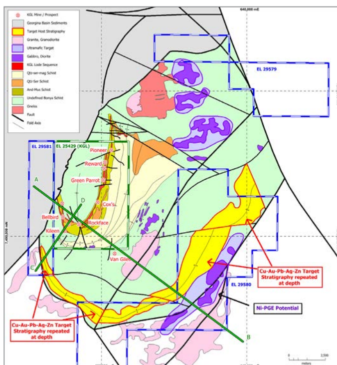
Figure 8 Interpreted geology of Jervois Domain project, Northern Territory.
