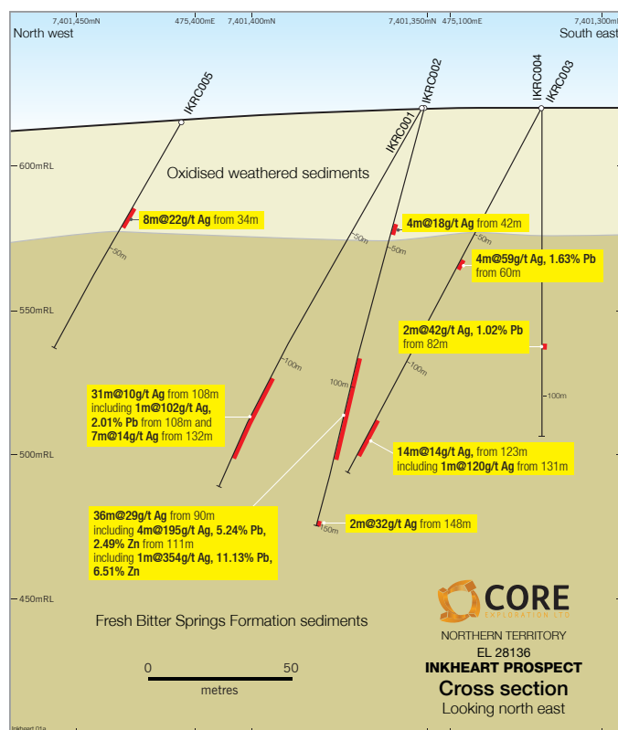
Figure 4 Inkheart drill results.
