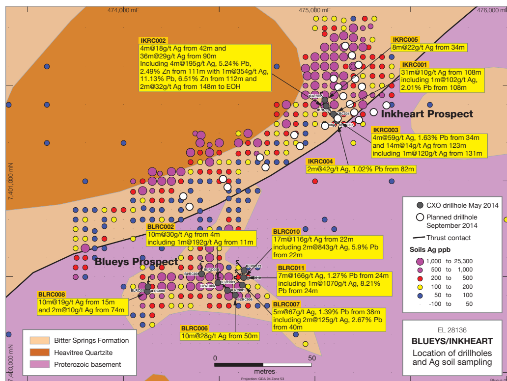
Figure 3 Blueys's drill results.
