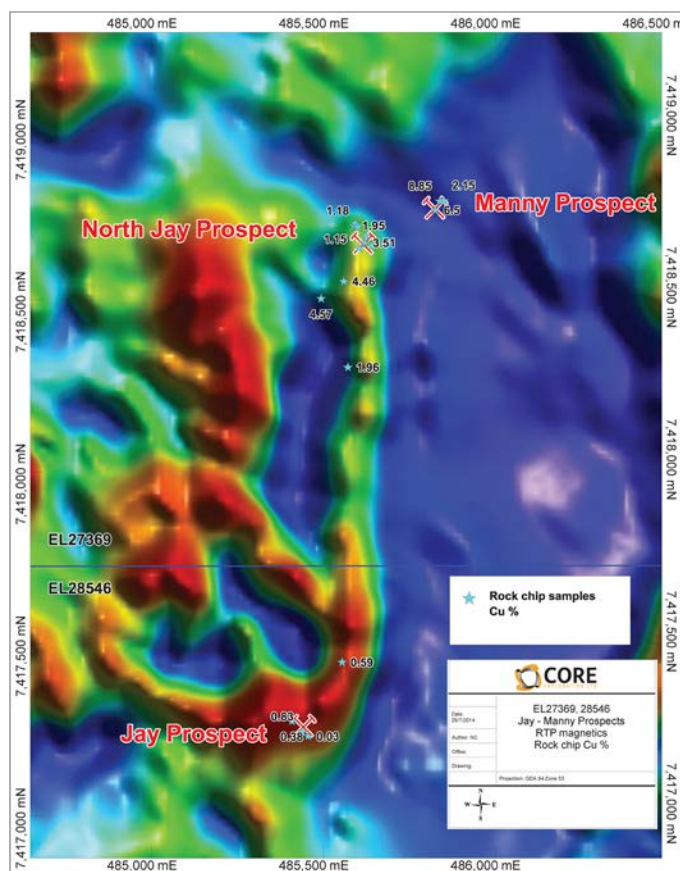
Figure 12 RTP magnetics and rock chip Cu%, Jay and Manny Prospects, Northern Territory.
