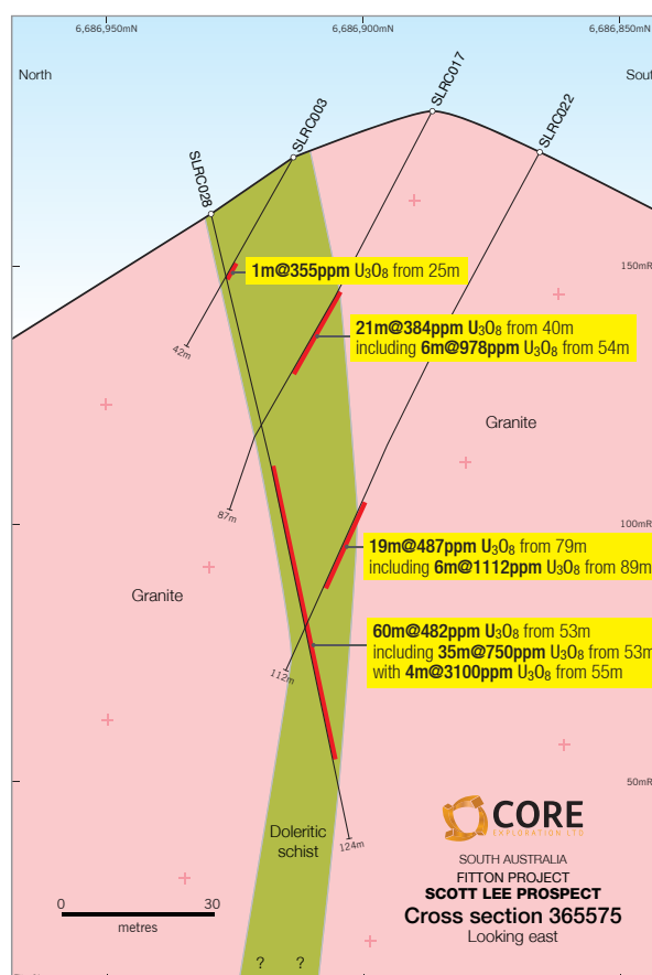
Figure 15 Cross section 365575, Fitton Project, South Australia.
