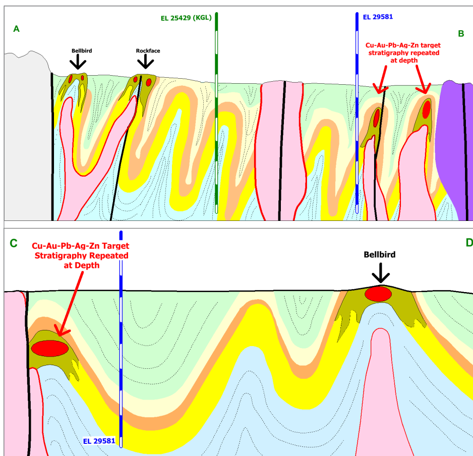
Figure 9 Cross sections A-B and C-D, Jervois Domain project, Northern Territory.
