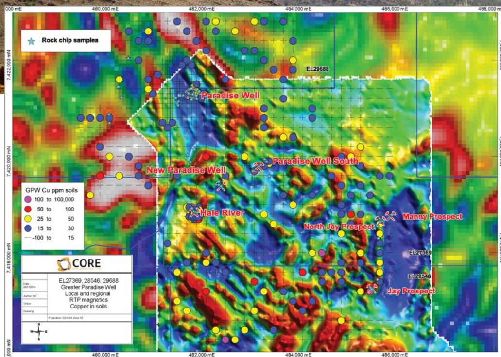
Figure 11 Local and regional RTP magnetics and copper in soils, Greater Paradise Well, Northern Territory.
