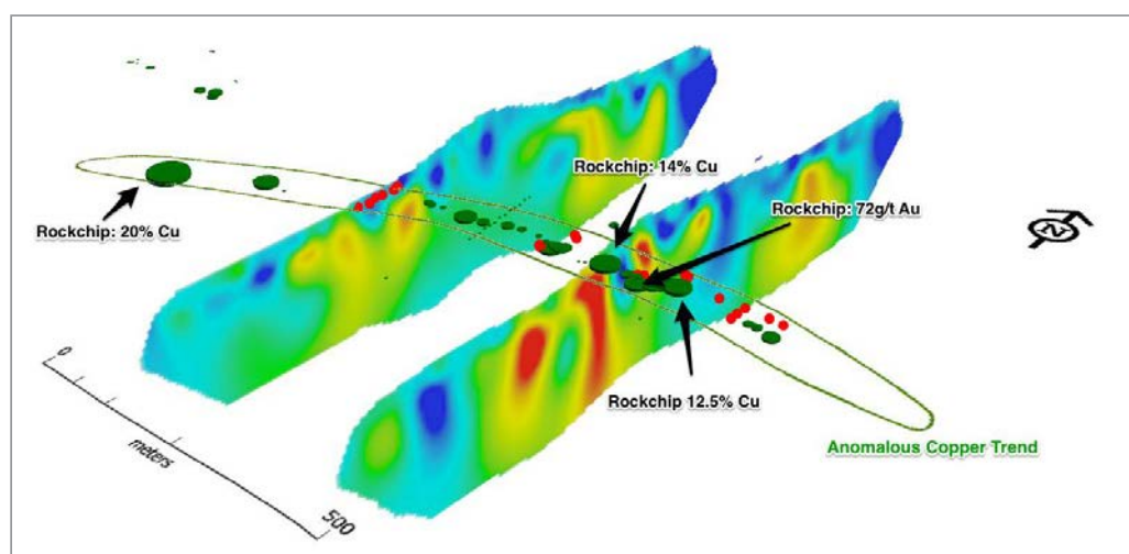
Figure 6 Copper Queen IP chargeability sections showing historic drilling (red) and thematic copper rockchip sampling (green).
