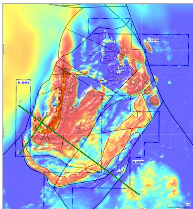
Figure 10 RTP magnetics over Jervois Domain project, Northern Territory.
