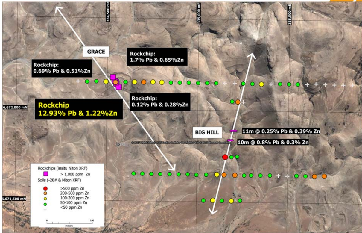
Figure 1. New soil and rock-chip results (XRF), previous channel sampling (XRF) and interpreted Grace and Big Hill shear zones, EL 5015, Yerelina.
