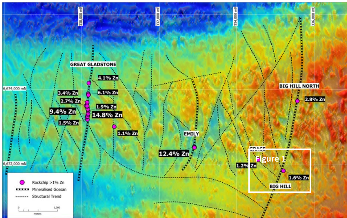
Figure 2. Multiple mineralised shear zone and interpreted to be repeated over 8km wide area overlain on magnetic image, EL 5015 Yerelina.
