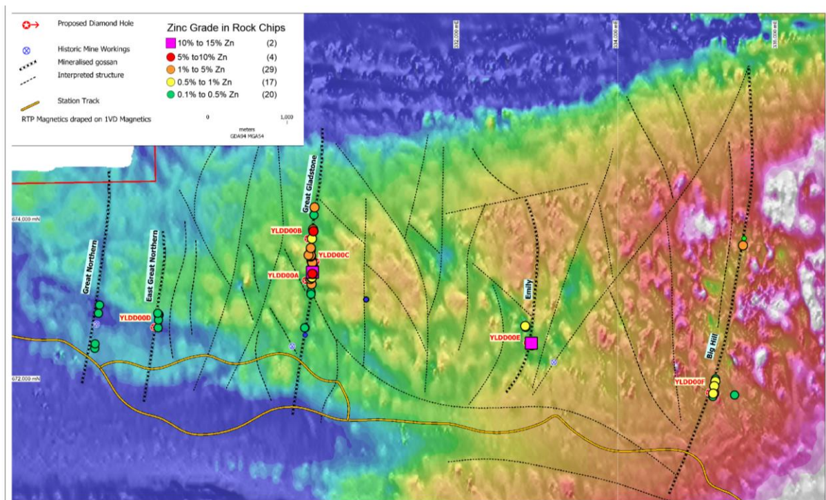
Figure 1. RTP Magnetic Imagery showing structural interpretation and zinc grade in rock chips.
