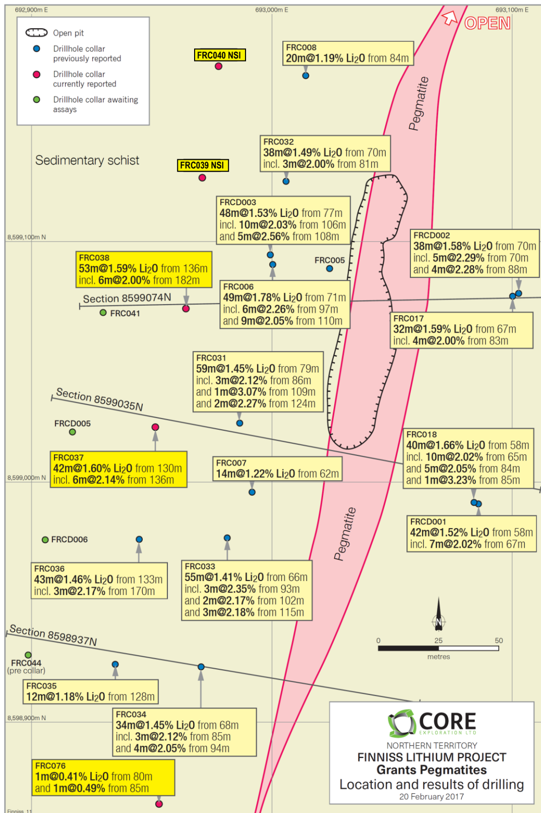
Figure 1. All RC and Diamond Drilling intersections and collar locations, Grants Prospect, Finiss Lithium Project, NT.
