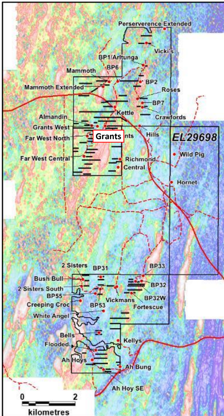
Figure 6. Pegmatite drill targets proximal to Grants overlain on new magnetics (left) and large-scale regional pegmatite drill targets (right), Finnis Lithium Project NT.
