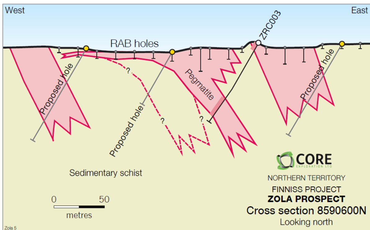
Figure 2: Cross section 8590600N of pegmatites intersected in drilling, Zola Prospect
