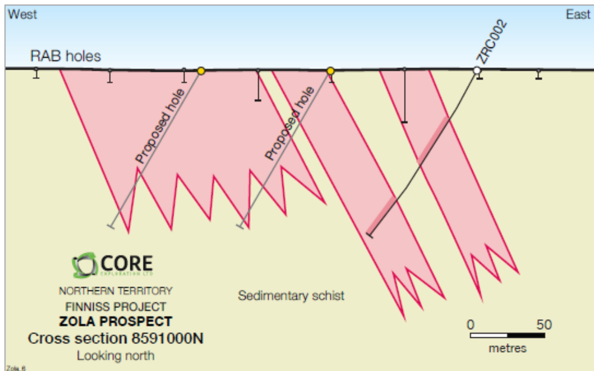
Figure 1: Cross section 8591000N of pegmatites intersected in drilling, Zola Prospect.
