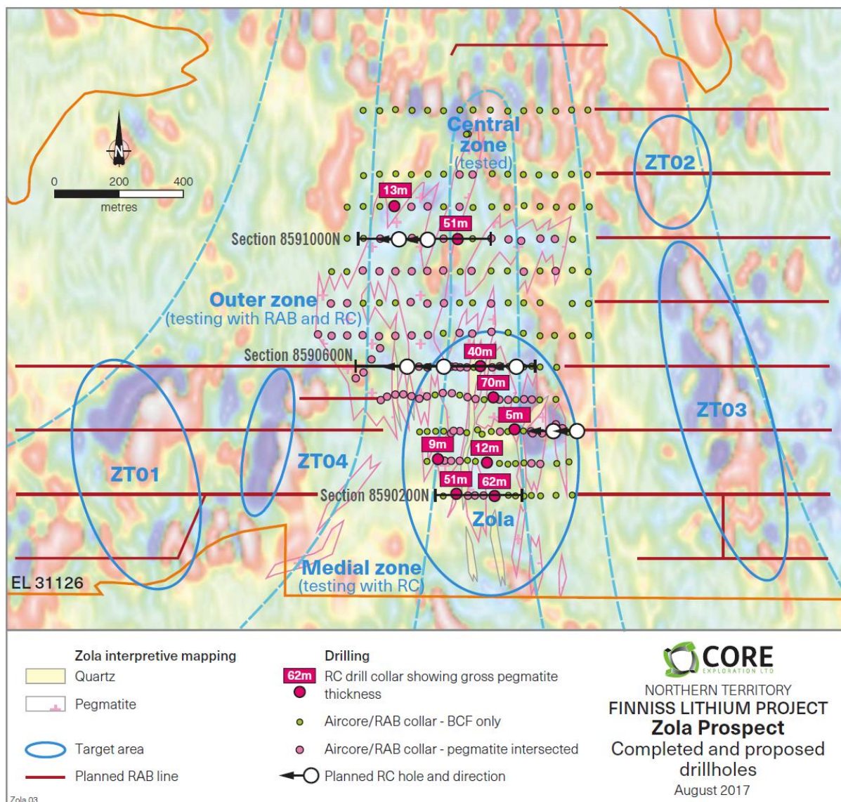
Figure 3: Recent and planned drilling, interpreted pegmatite geology and drill targets overlain on magnetic image at Zola Prospect.
