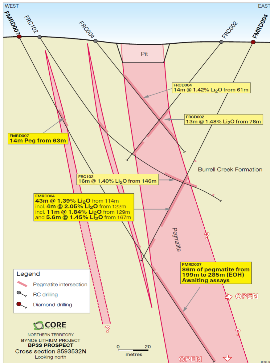
Figure 1. Drill cross-section at southern BP33.
