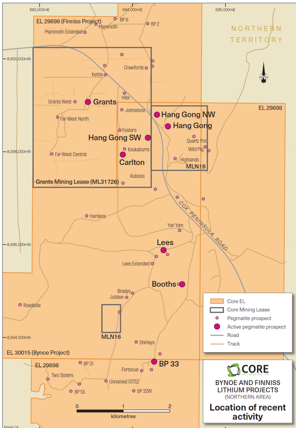
Figure 3. Recent exploration and drilling at pegmatite prospects within the Finnis Lithium Project near Darwin in the NT.
