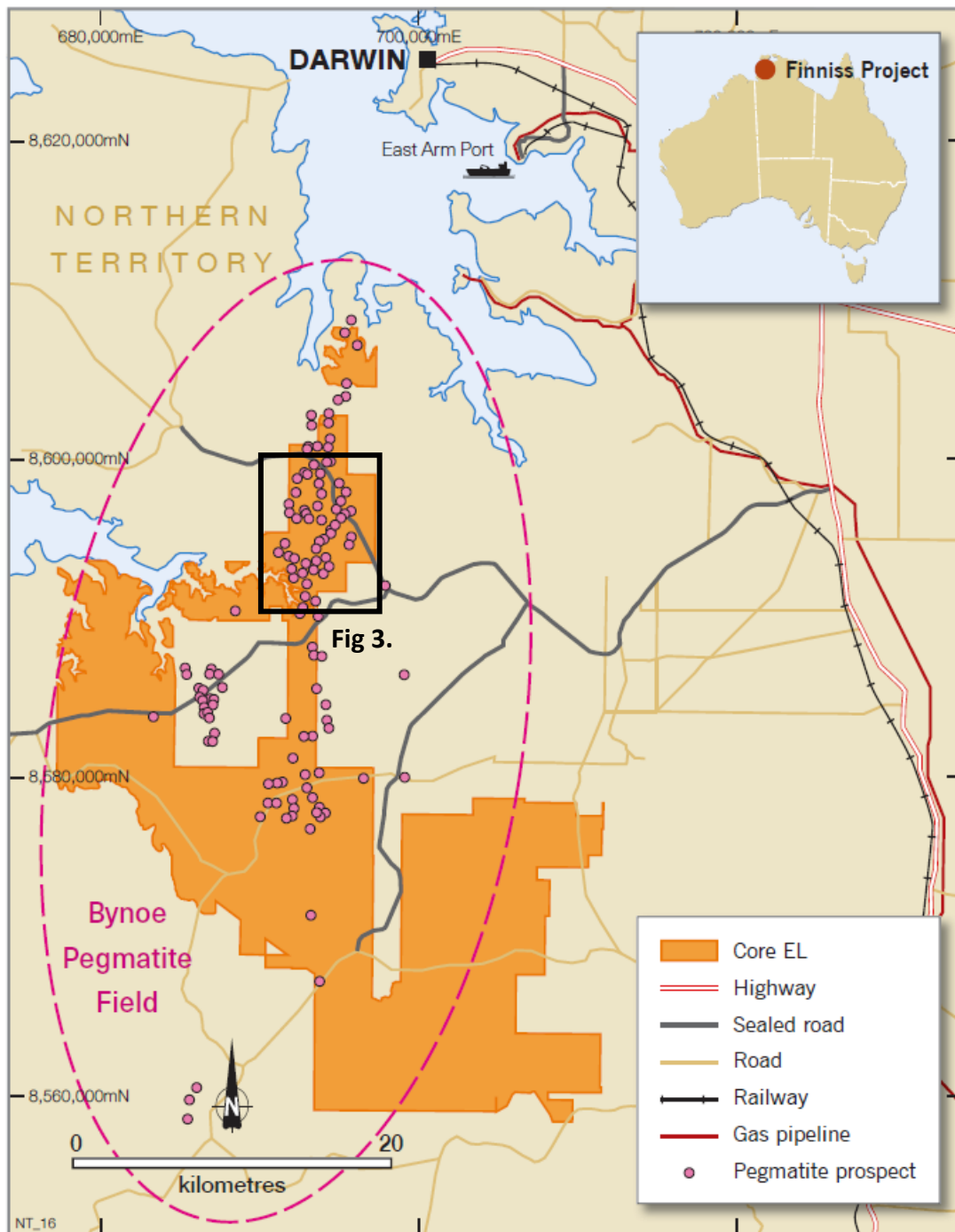
Figure 4. Pegmatite prospects within the Finniss Lithium Project near Darwin, NT
