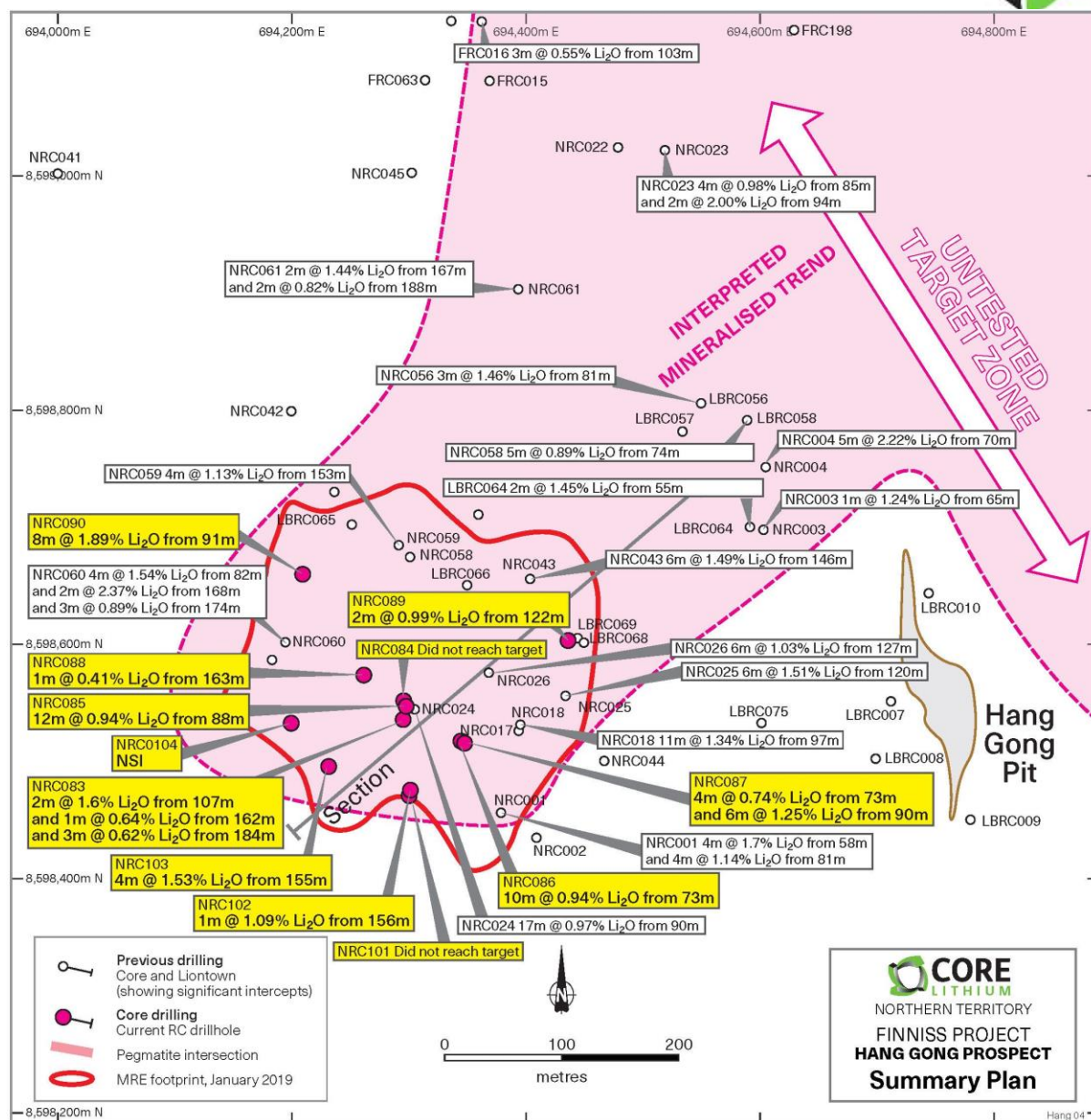
Figure 3. RC drilling results in the greater Hang Gong area, highlighting recent assays results
