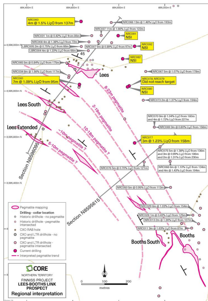
Figure 1. Recent RC drill intersections at Lees-Booths Link Prospect
