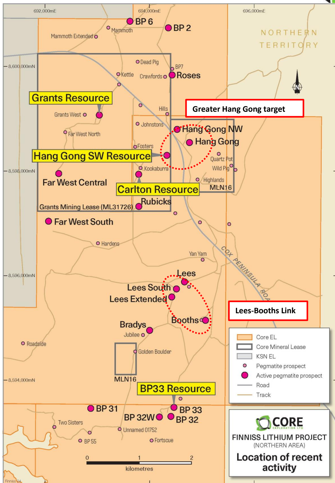
Figure 4. Active pegmatite prospects in the northern area of Finnis Lithium Project.
