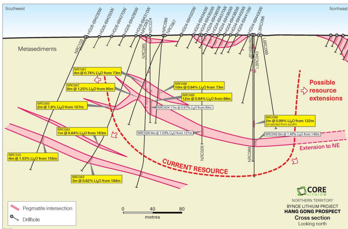
Figure 2. Recent RC drill intersections at Hang Gong Prospect in section
