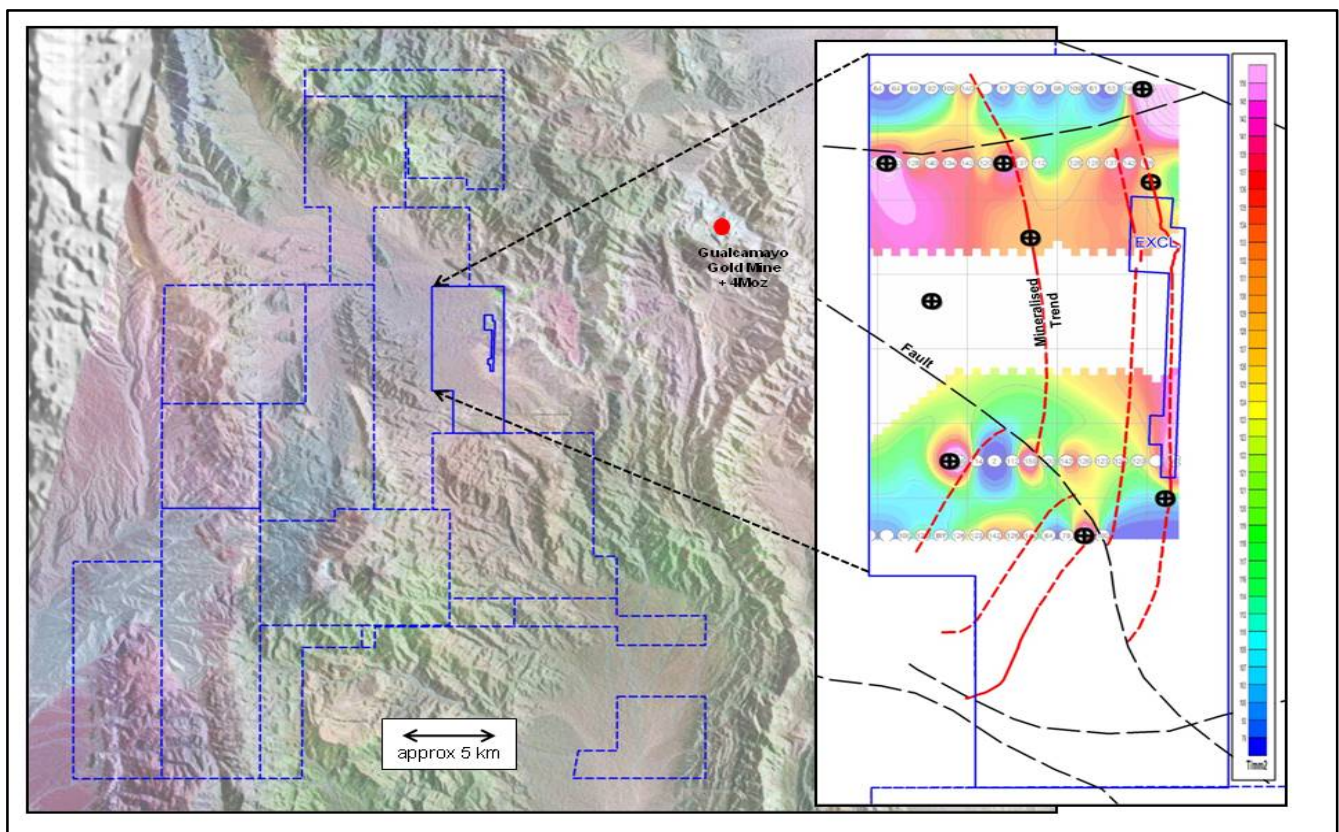
Fig1: Satellite image showing project area & insert of preliminary radon cup sampling, interpreted geological features & proposed drilling (crossed circles).
