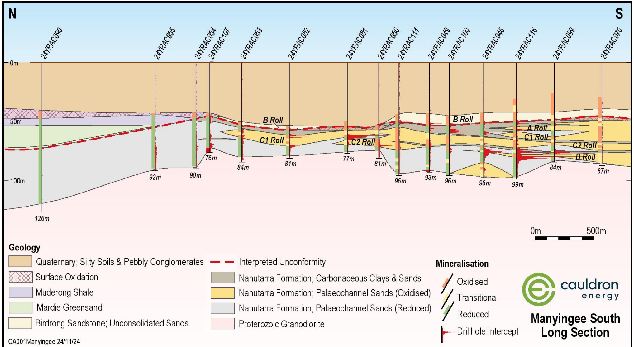
Figure 5. Revised Manyingee South Long-Section.
