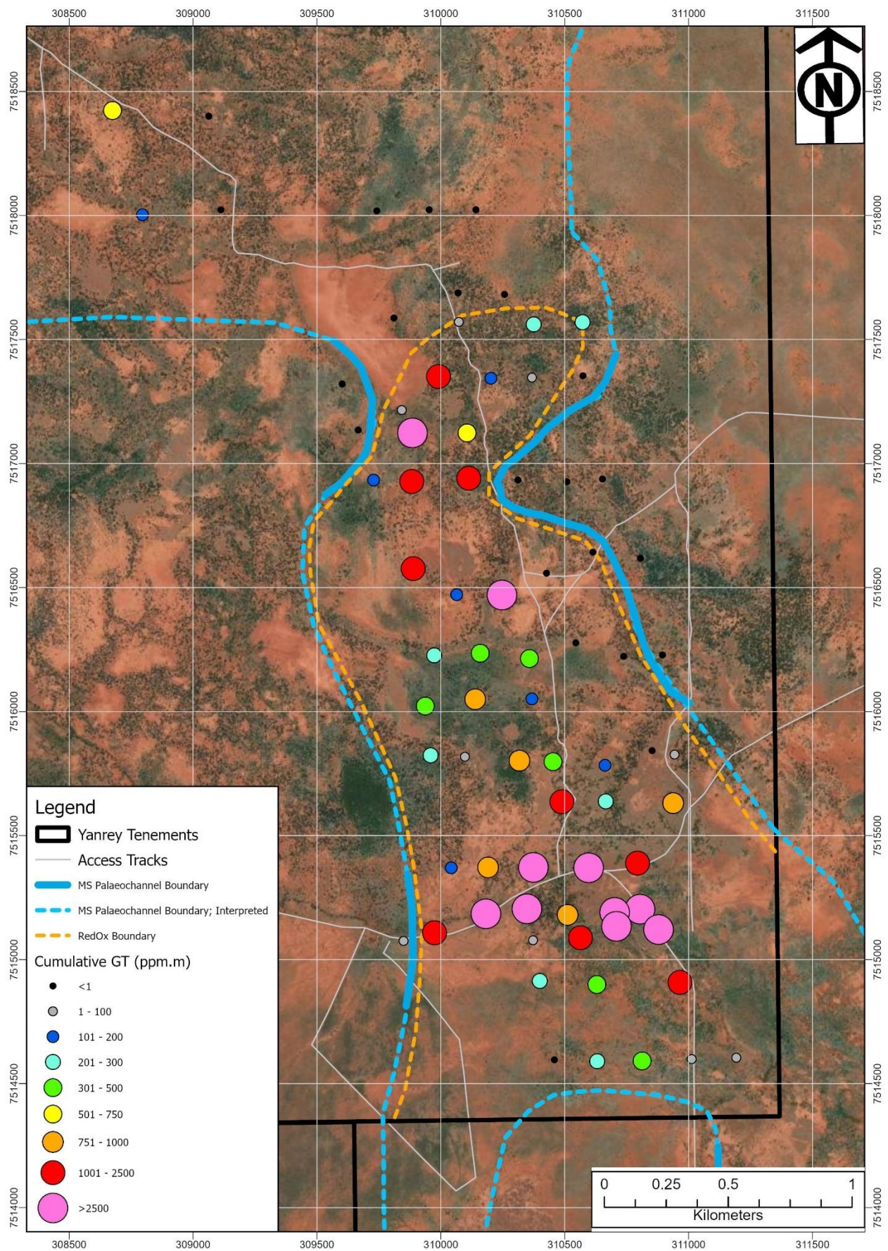
Figure 4. Manyingee South Uranium Prospect – grade thickness (GT) map. Note the high-grade zones in the north and south associated with the closure of the C and D rolls respectively.
