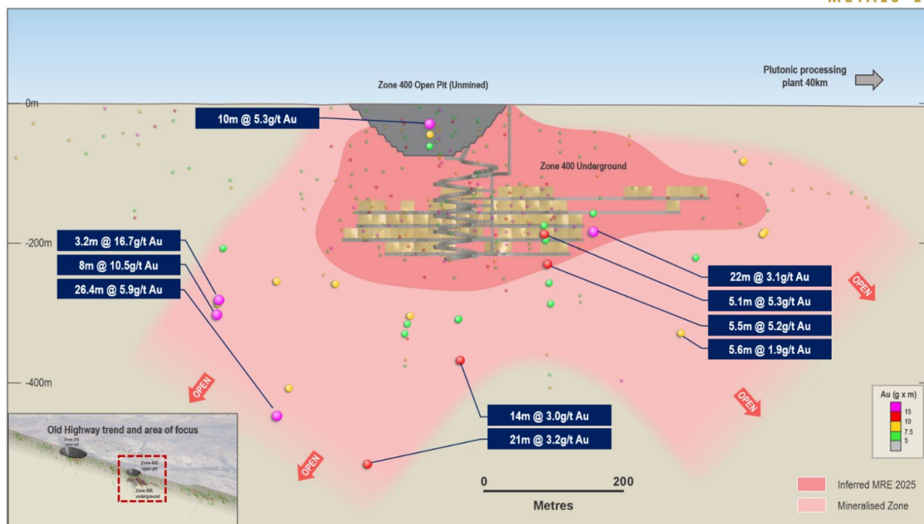
Figure 1: Old Highway Zone 400 open pit and underground deposit showing new drilling results
