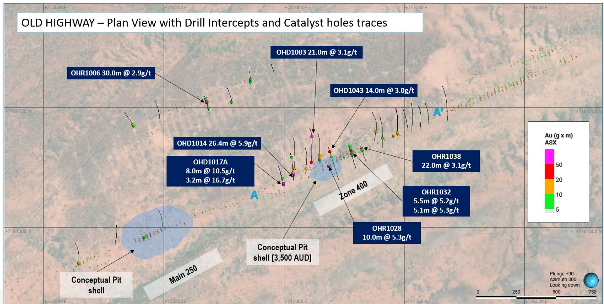
Figure 4: Old Highway plan view with drill intercepts and Catalyst traces
