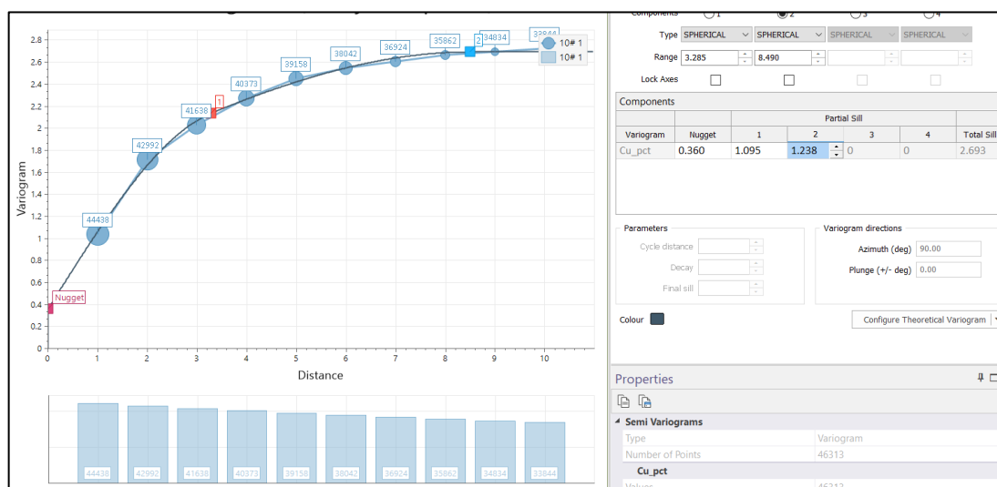
Figure 4-5: FWS downhole variogram
