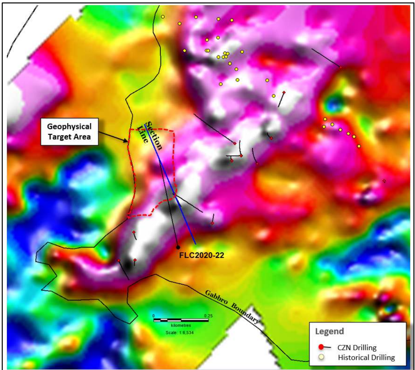
Figure 4 – Fraser Lake Complex – IP Chargeability Image Showing the Matrix Trend (high IP chargeability anomaly), Target Area, Past Drilling and Figure 3 Cross-Section Location (Plan Location Shown in figure 2)
