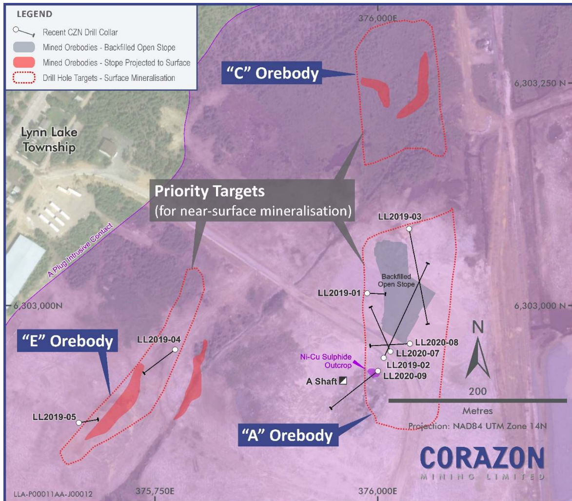
Figure 1 – Drill hole location plan, with mined deposits (“Orebodies”) and target areas in the northern part of the Mining Centre (refer to Figure 2 for location).
