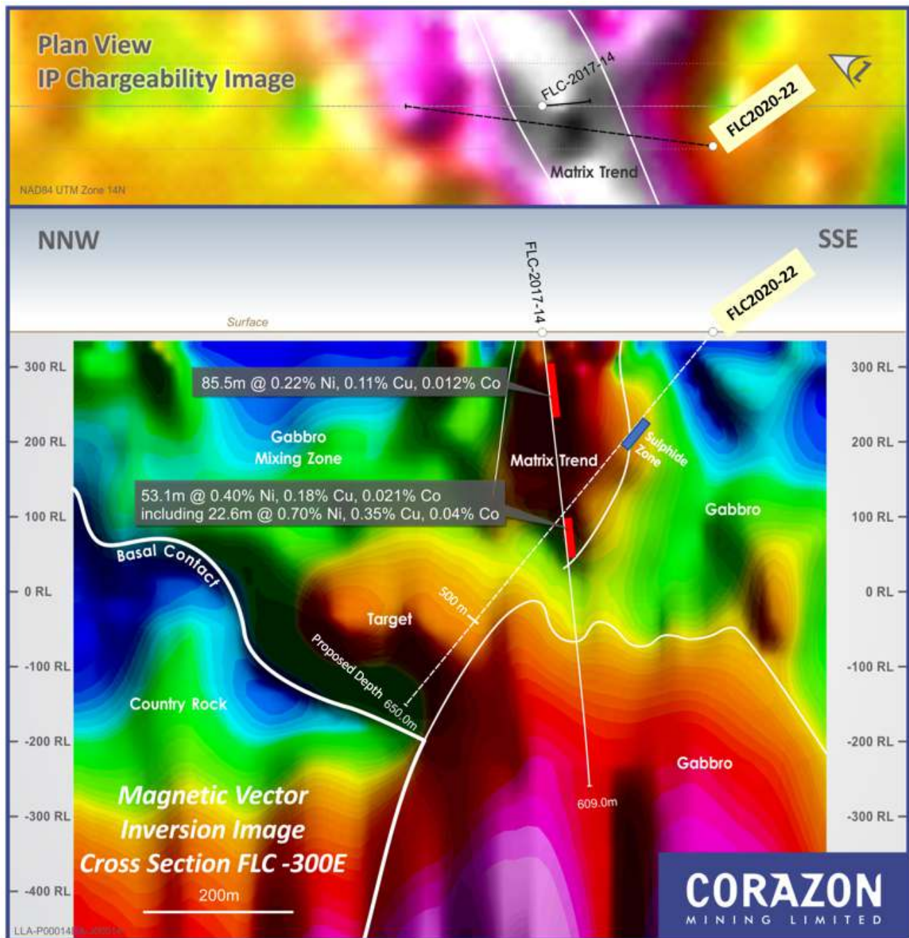
Figure 3 – Cross-section and Plan Geophysical Images for Hole FLC2020-22, with Past Drilling and Results (refer to Figure 4 for section location)
