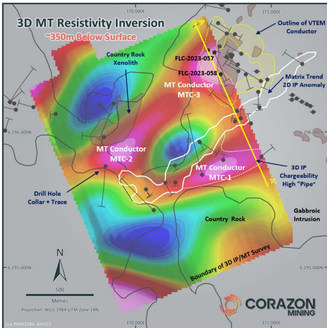
Figure 1 – MT Resistivity Inversion Image at ~350m below surface. Hot colours depict strong conductivity. “MTC” targets and drill holes FLC-2023-057 and -058 are located on this plan. The location of the MT geophysical survey area within the Lynn Lake Project is shown in Figure 4. The section line (A-A’) for Figure 2 is also identified.
