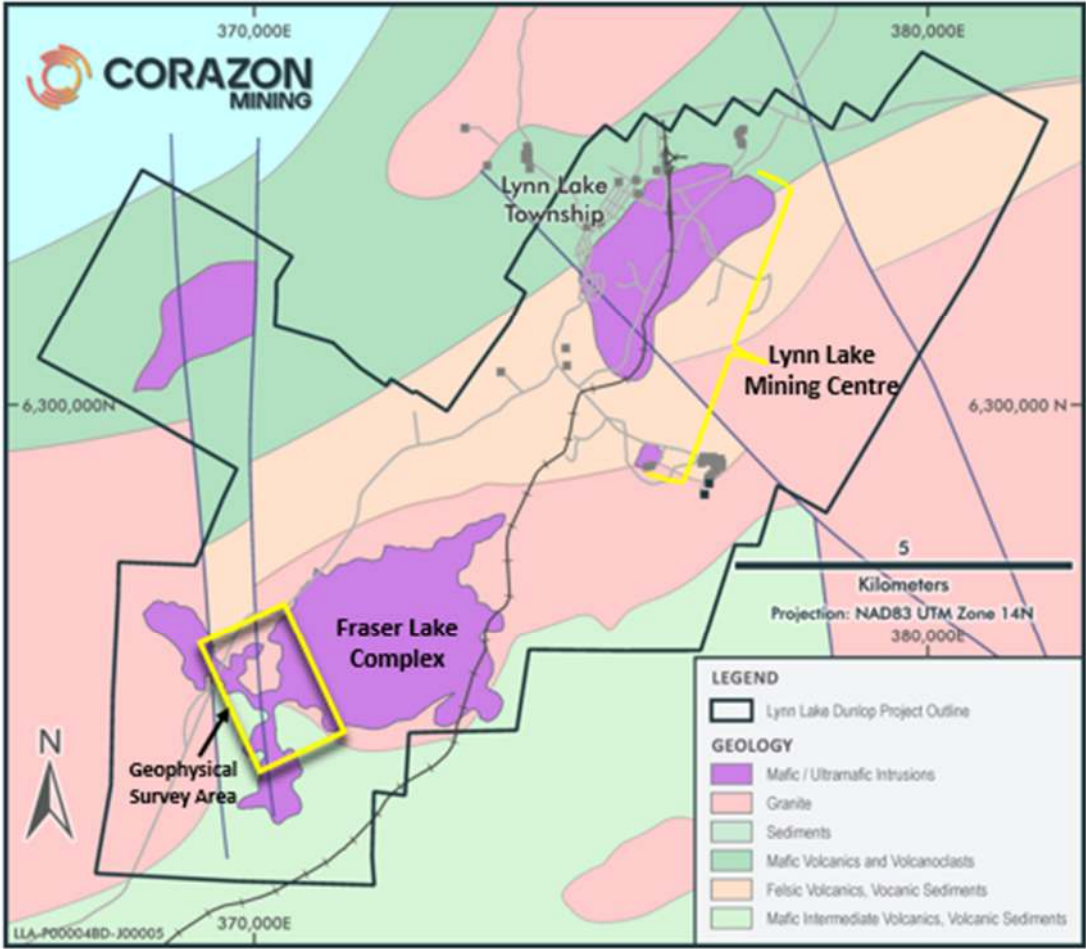
Figure 4 – Lynn Lake Project – Interpreted geology and 3D DCIP and MT survey area defined.
