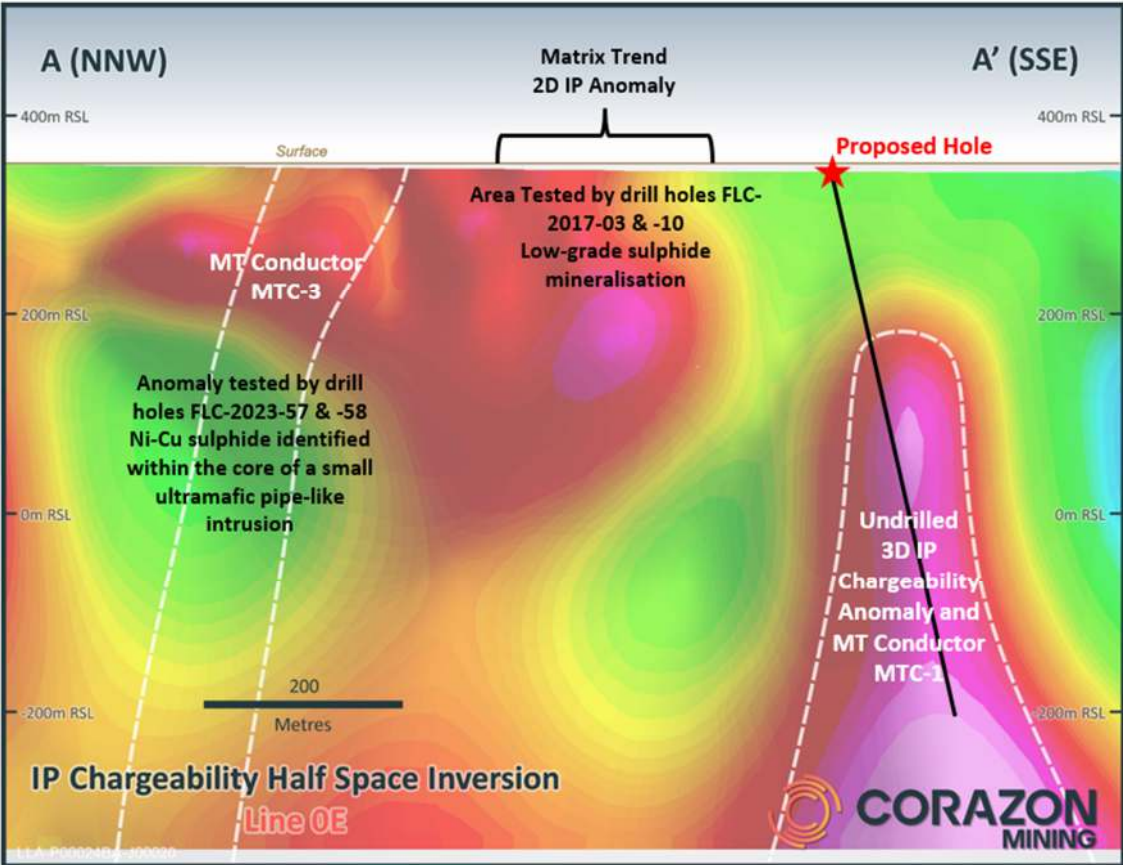
Figure 2 – IP Chargeability Cross-Section Image at section line A-A’ (see Figure 1). Hot colours depict strong IP chargeability, potentially indicative of disseminated sulphides. The outlines of MT conductive bodies MTC-1 and MTC-3 are superimposed on this image.
