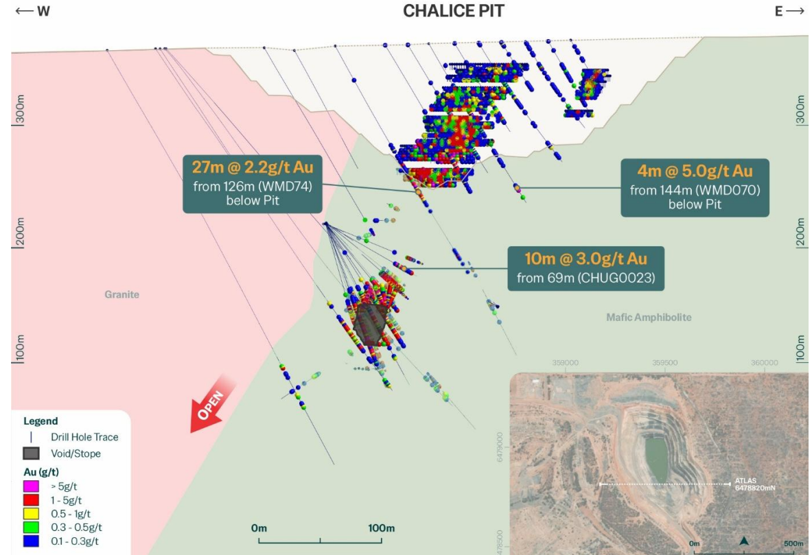
SECTION VIEW LOOKING NORTH (+/-10m) ATLAS 6478820mN
