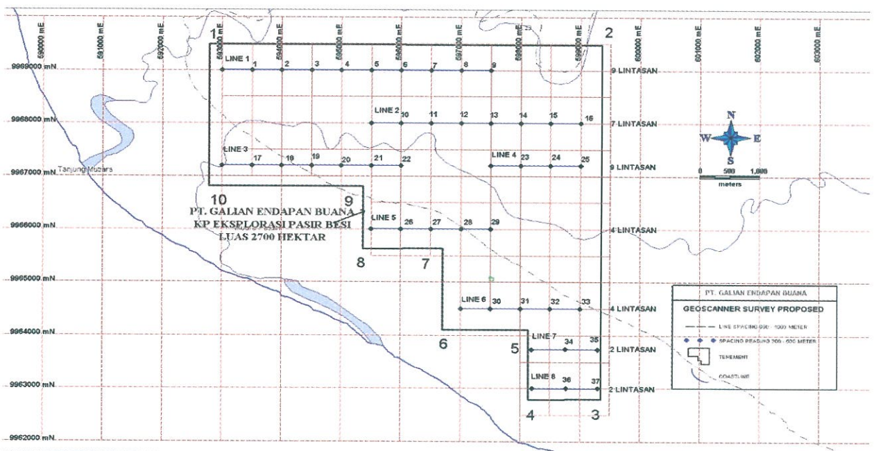
Agam Tenement 2 proposed eight lines of ground EM survey
