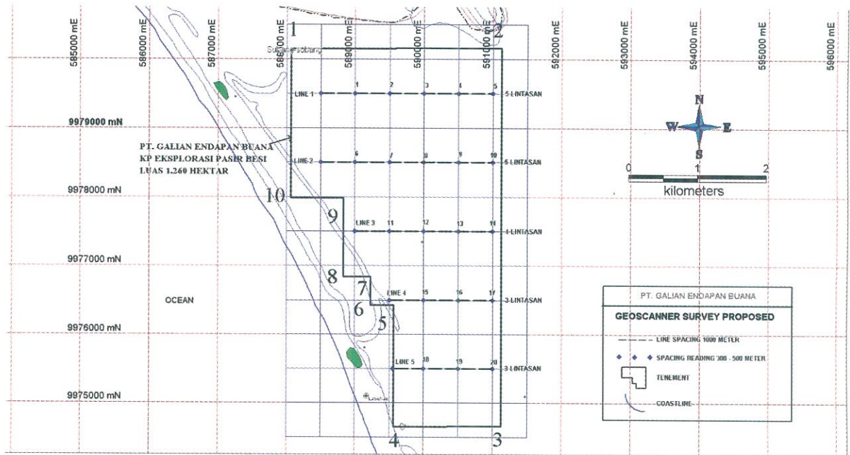
Agam Tenement 1 proposed five lines of ground EM survey
