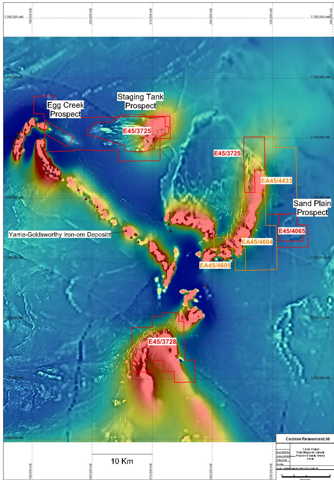
Fig 7. Regional setting of the Yarrrie Project overlain onto the magnetic intensity with the most intense responses attributed to the Nimingarra Iron Formation.
