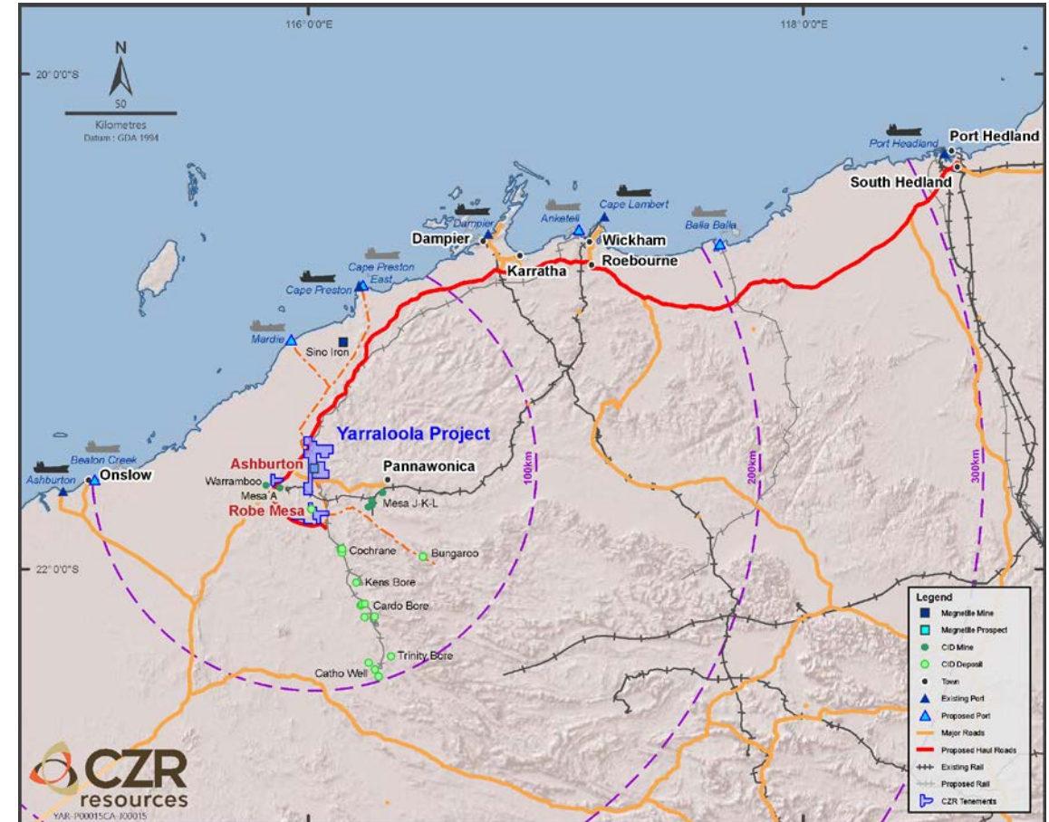
Location map for the Robe Mesa on the Yarraloola project in the West Pilbara, RioTinto operated mines (Warramboona, Mesa's A and J-K), other significant CID deposits in the region and the current and proposed transportation options in the region.
