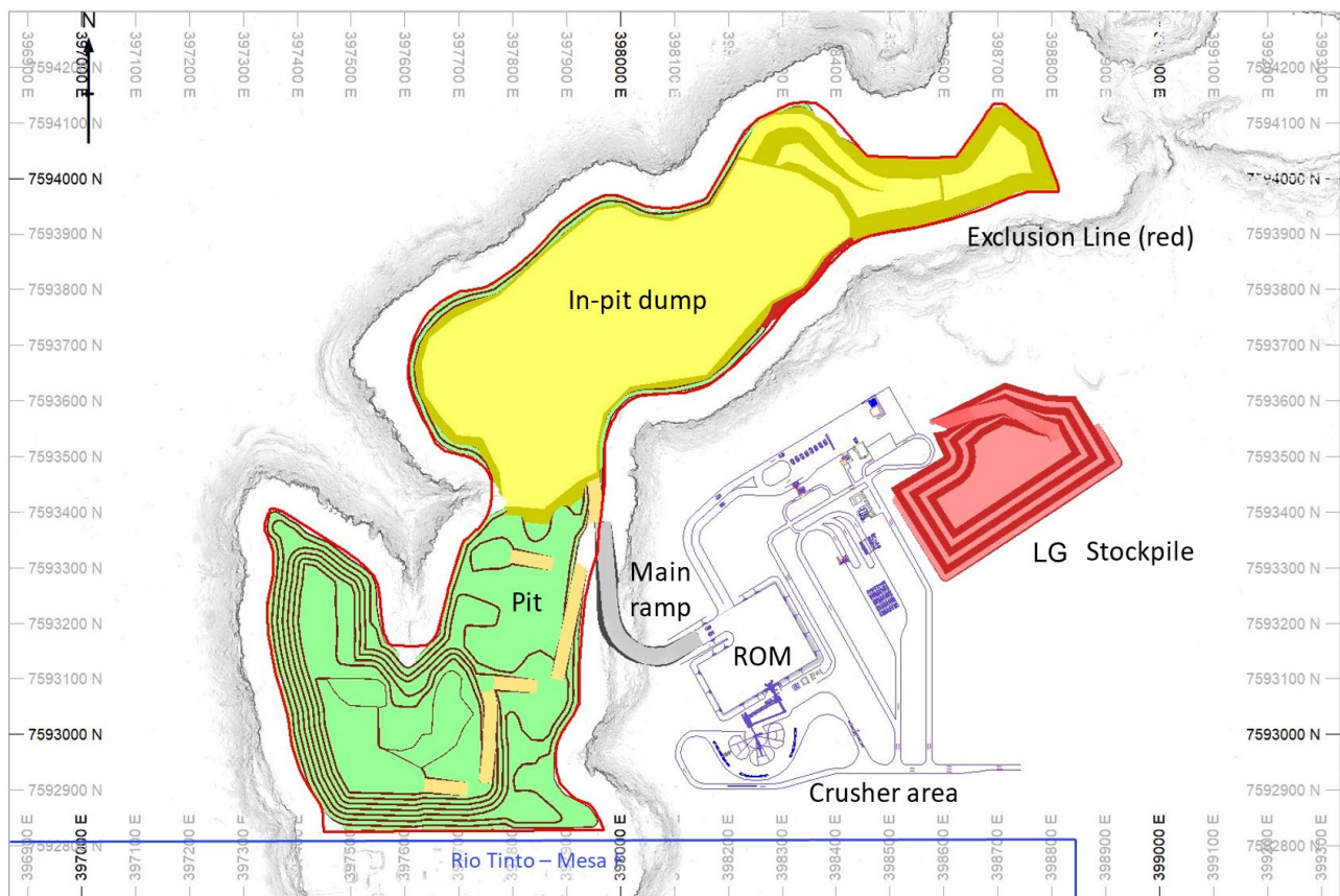
Figure 3. Robe Mesa Site Layout – Final pit with in-pit waste dumps, mine operations centre (MOC), processing plant and LG stockpile
