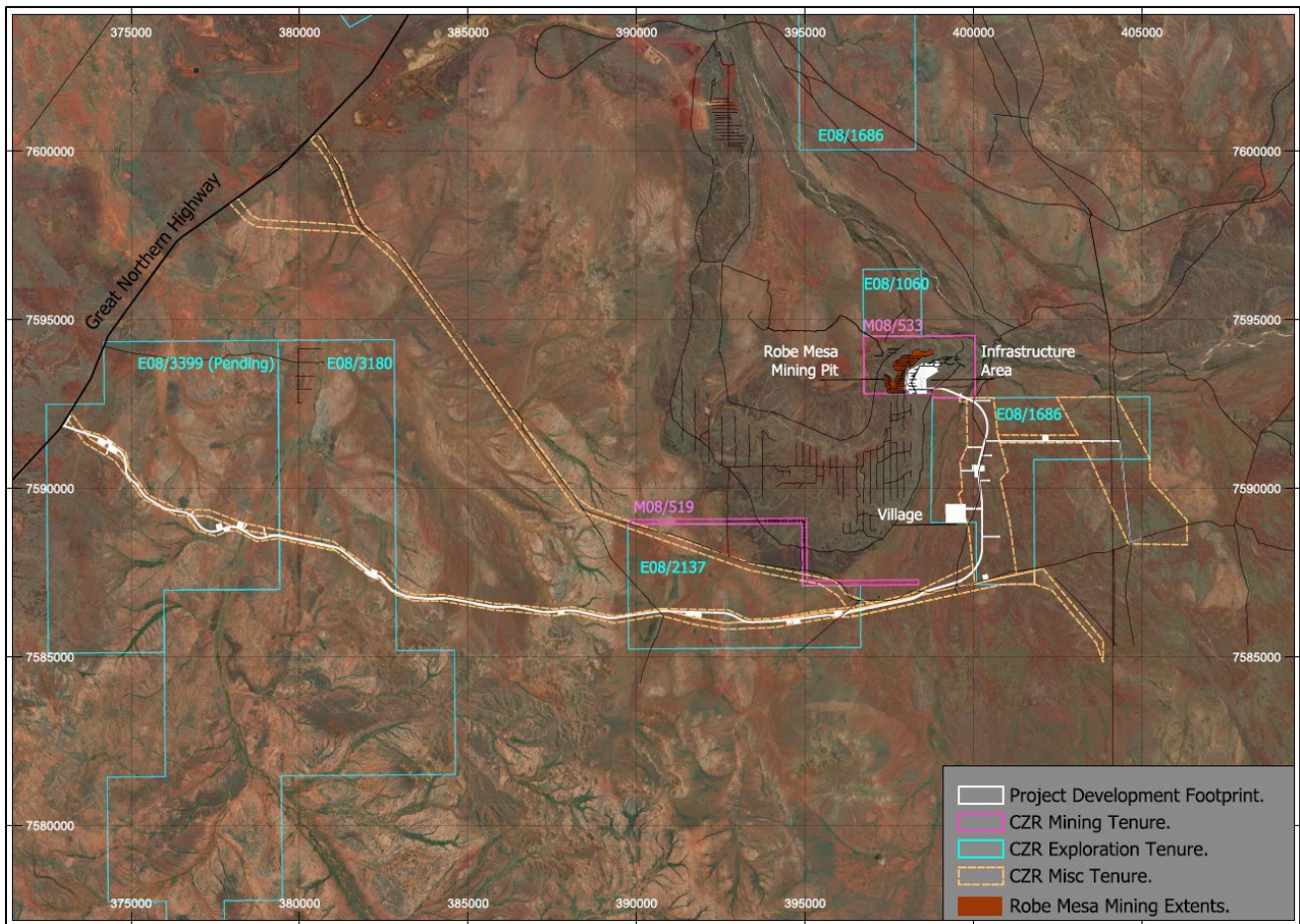
Figure 4. Robe Mesa Project Layout – Including designed haul road, village and tenure
