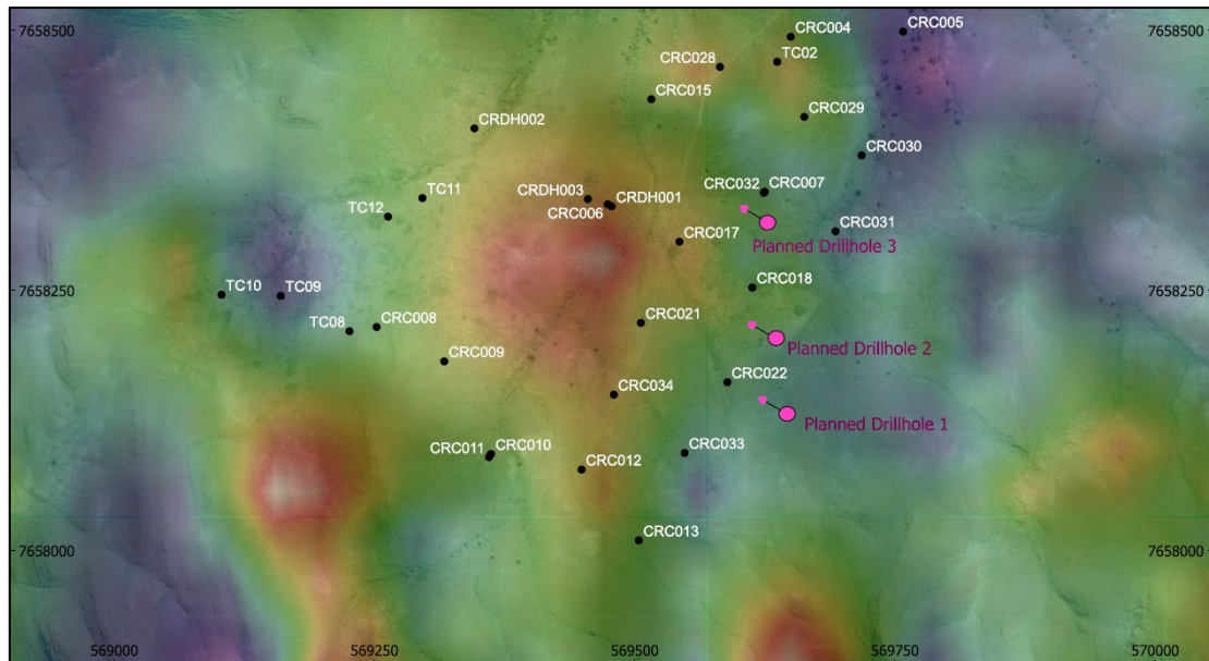
Figure 8. Top Camp Gravity survey – existing drill holes and planned drill holes
