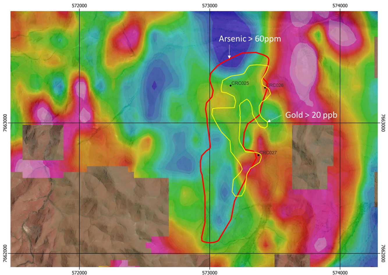
Figure 10. Bottom Camp Gravity image with gold and arsenic surface geochemical anomalies
