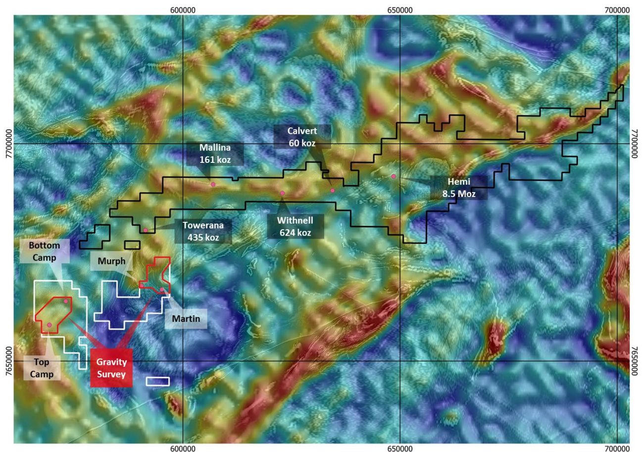
Figure 6. CZR's Croydon project and De Grey Mining's Hemi Gold Project – Regional gravity over magnetics
