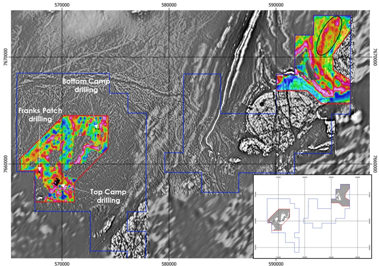
Figure 7. Preliminary Croydon ground based gravity results over regional magnetics – insert shows completed gravity stations within planned survey area
