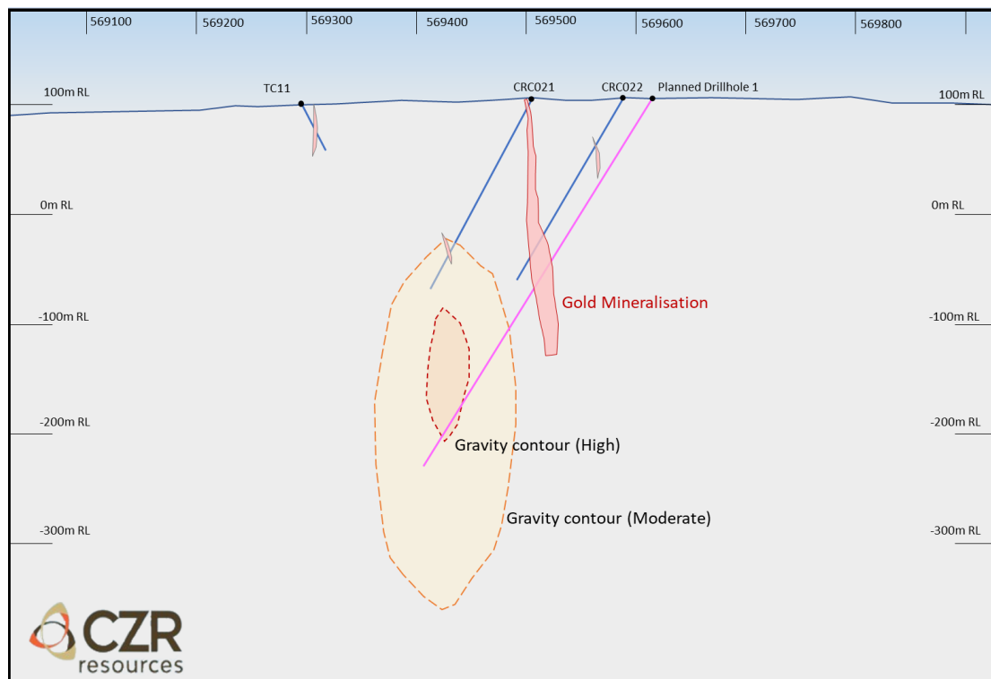
Figure 9. Top Camp Gravity inversion model – intrusion-related golds target (gravity high) with existing drill holes, primary gold mineralisation and planned drill hole
