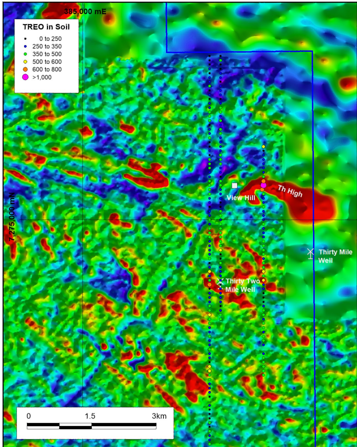
Figure 2: TREO ppm on radiometrics Th (note coincident large Th anomaly with >800ppm TREO anomaly).
