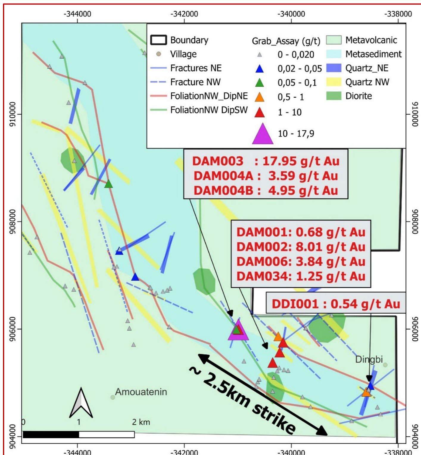
Figure 4. Interpreted Geological map of the northern part of the tenement with Assay results.
