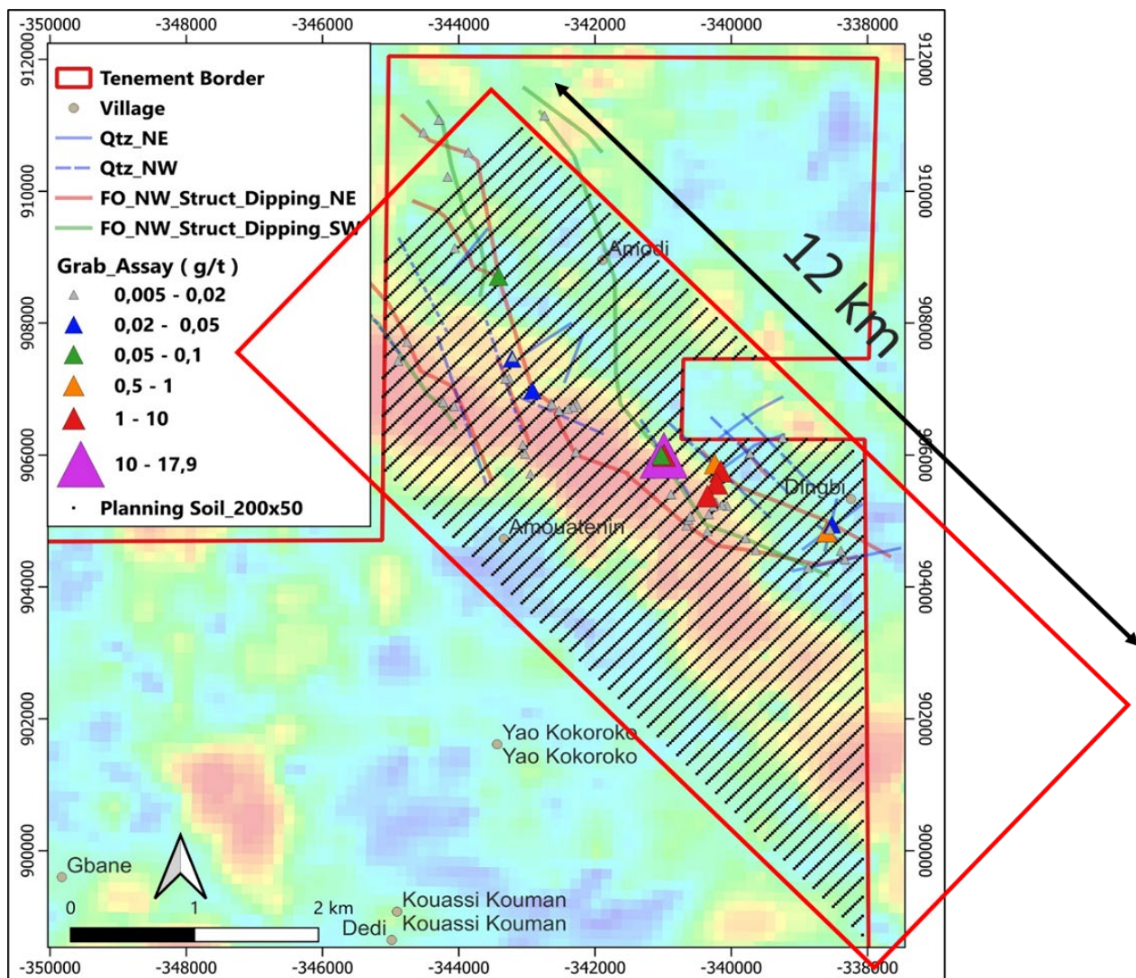
Figure 6. Plan map of soil geochemical program.
