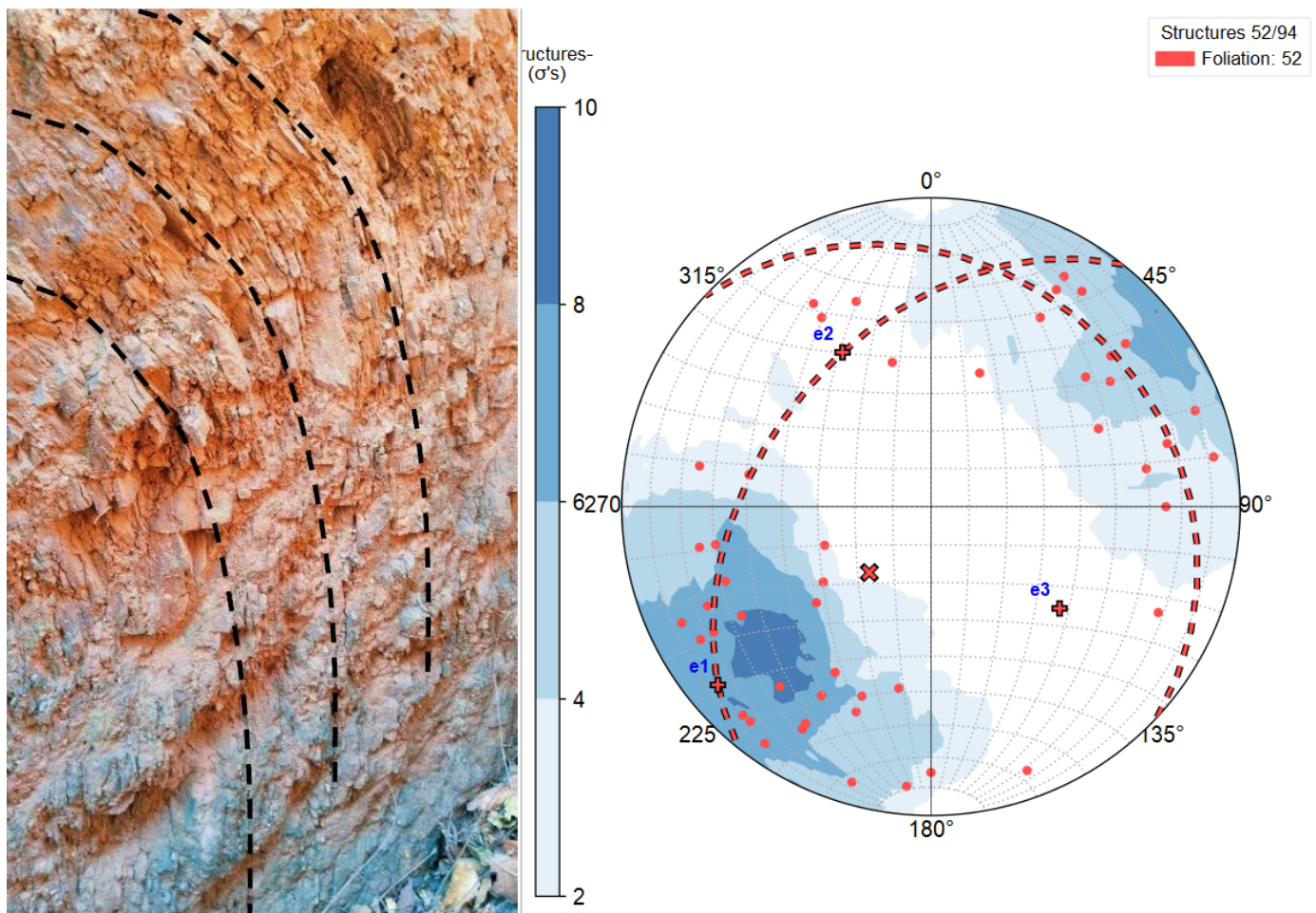
Figure 5. anticline fold observed on old tranche and stéréonet of the foliations in northern part of tenement.
