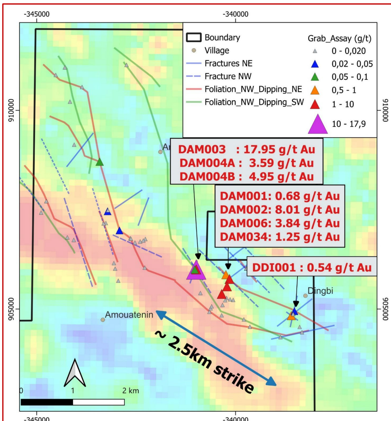
Figure 3. Plan map showing location of Rock-chip sampling results highlighting gold anomalous zones on Aeromagnetic image and mapped artisanal workings.
