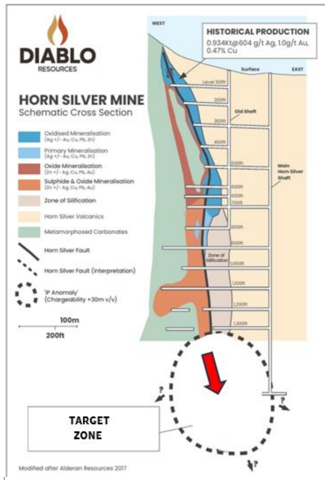
EAST-WEST VIEW
