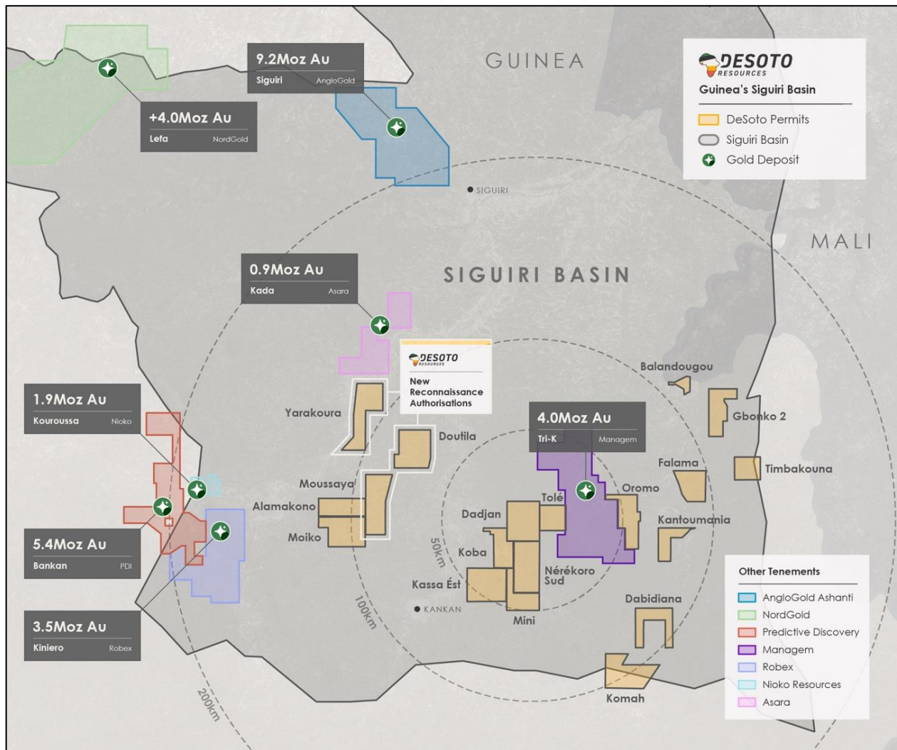
Figure 3 - DeSoto Resources' Siguiri Basin Portfolio, with Koba part of its south-central Siguiri Project block, which sits directly abutting Managem's 4Moz Tri-K Deposit.
