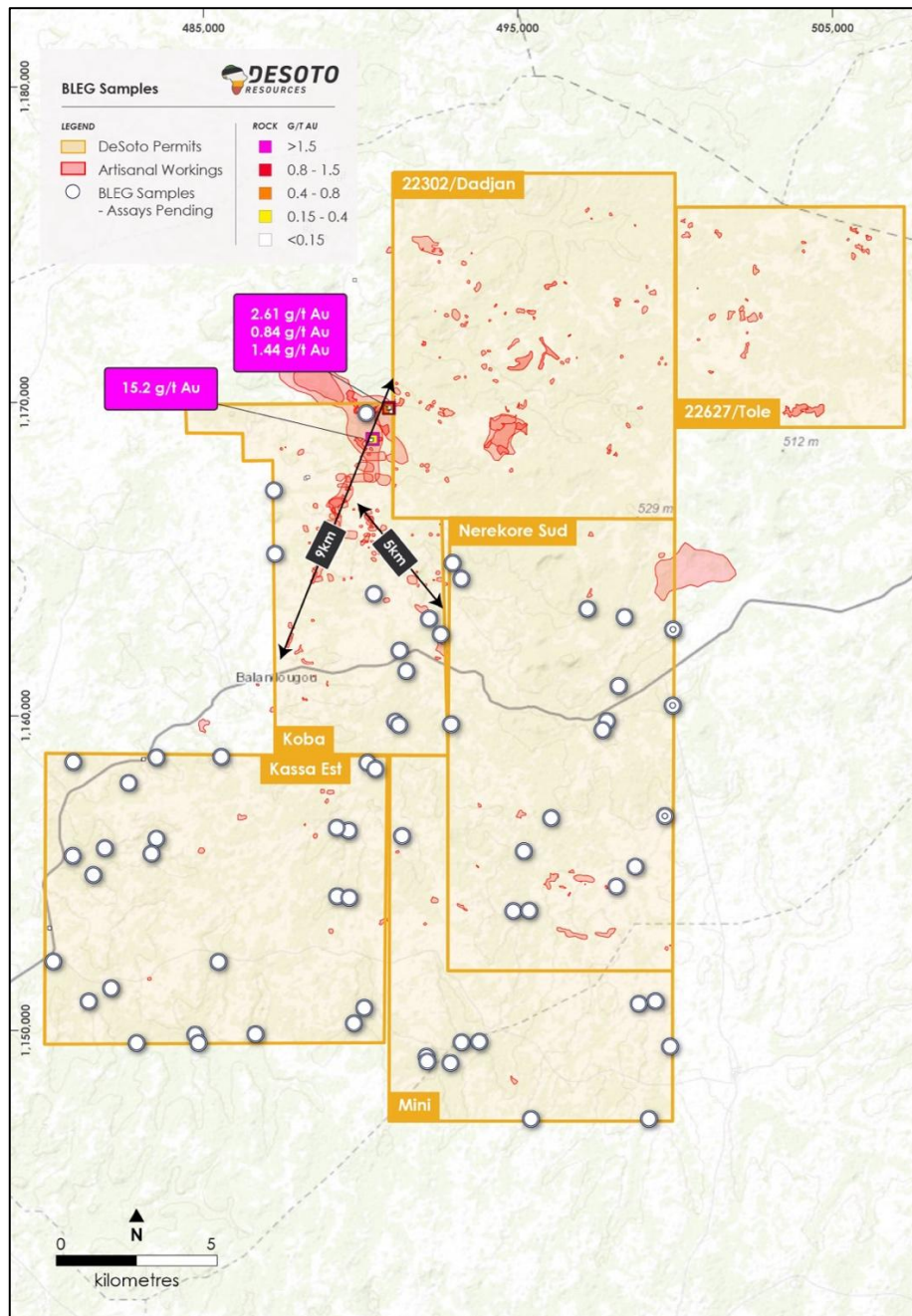
Figure 2 – DeSoto's south-central Siguiri Projects, including Koba, Dadjan, Tolé, Nerekore Sud, Kassa Est and Mini, with the regional BLEG program and dump samples overlain mapped artisanal workings, highlighting the 9km-long zone at Koba and its structural interconnection with Dadjan and Nerekore Sud.
