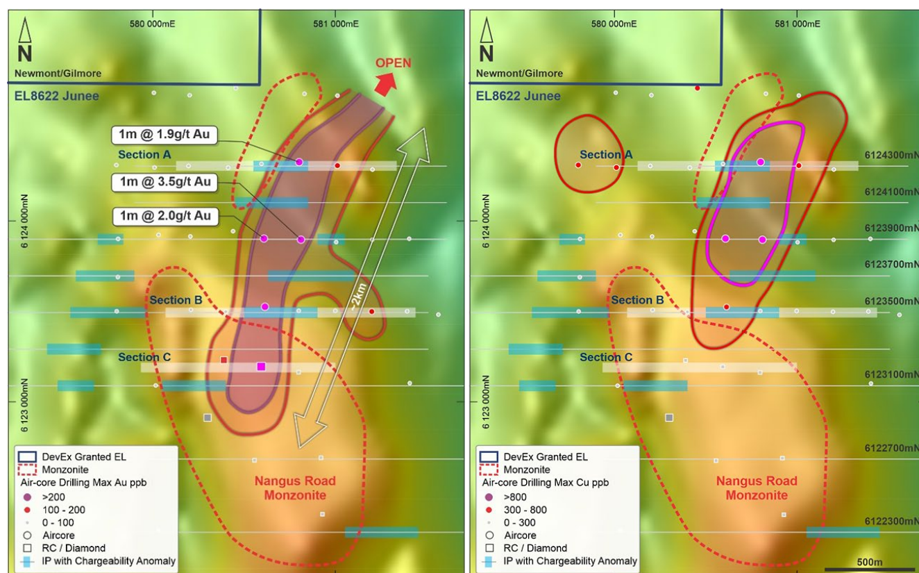
Figure 6: Nangus Road Prospect at Junee – Recent broad-spaced (400mN x 200mE) air-core + RC drilling, bedrock copper and gold anomaly (maximum Au and Cu assay per hole), peak assay of 1,410ppm Cu and 3.5g/t Au (3,490ppb Au), underlain by RTP magnetics. New IP Survey lines and anomalies are also shown. The copper and gold bedrock anomaly lies within and along the northern margin of the monzonite anomaly and remains open to the north.
