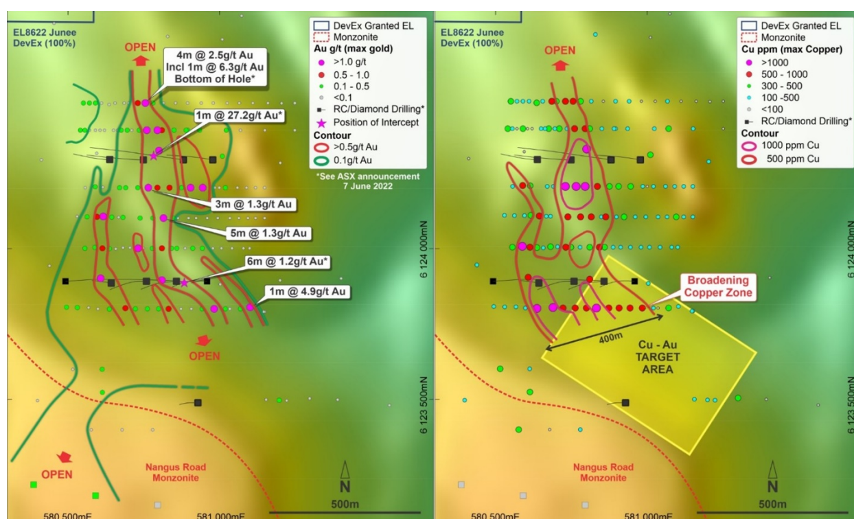
Figure 8a: Nangus Road Prospect showing location of current drill-holes. AC drilling has been thematically mapped to show maximum gold values down the hole.
