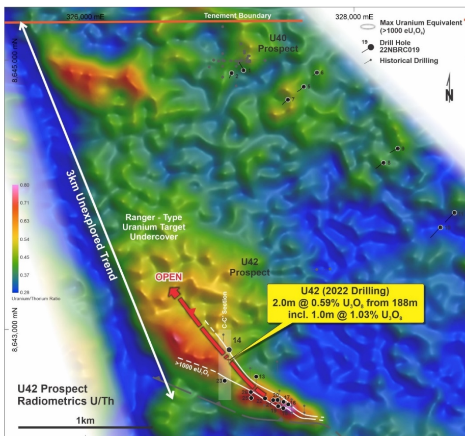
Figure 6: U42 Prospect – Airborne Radiometric Image for Uranium/Thorium trend, showing the location of hole RC14, which remains open for several kilometres to the north-west.
