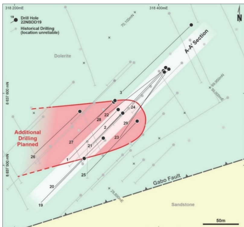
Figure 3: Nabarlek South Prospect – Drill-Hole Collar Plan.
