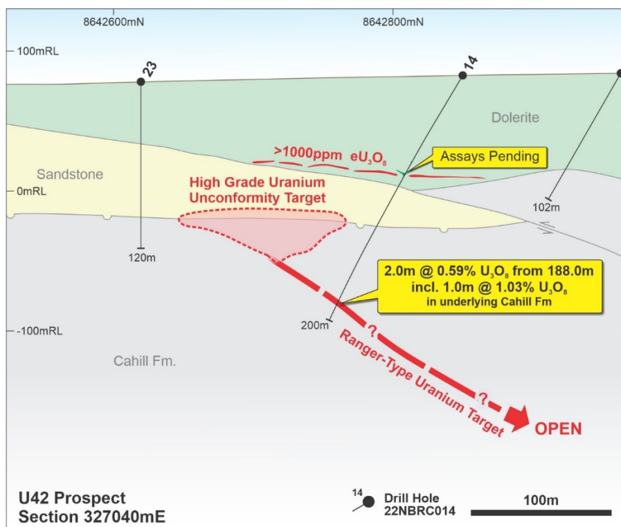
Figure 5: U42 Prospect – Cross-Section C-C' showing uranium mineralisation intersected in hole RC14.
