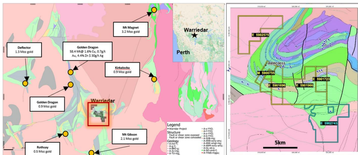
Figure 1: LEFT: Location of the Warriedar Project with respect to significant deposits/mines in the region, over regional bedrock geology (GSWA). RIGHT: a closer view of the Warriedar project, including the recently granted tenement to the southeast (see AWV ASX announcement 16 th September 2022). The drillhole annotated on the map (RRRC 0011) returned 20 m @ 2.12 g/t Au (see Appendix 1 and Red Dirt Metals ASX announcement dated 22nd June 2021).
