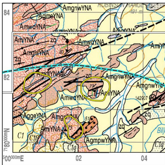
Mapped geology shows peridotite (a mantle derived rock often associated with Ni-Cu-PGE sulphide deposits) coincident with a magnetic anomaly and a strong conductor within a few 100 metres of the Craton margin. The conductors may be caused by economic metallic sulphides. These new targets are prioritised for ground EM and drill testing
