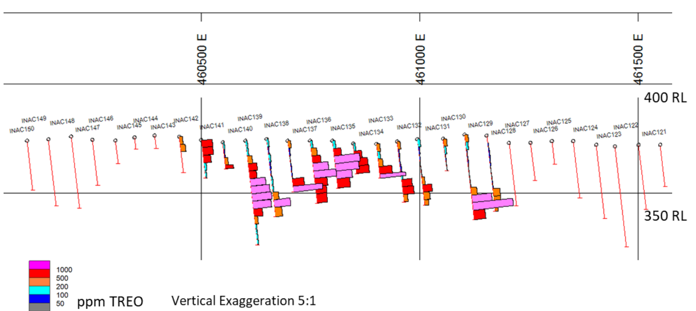
Figure 2. Total Rare Earth Oxides from two sections of assays received to date. Red drill traces = assays not yet received. TREO intersections within the clay appear to be thick and relatively continuous from the limited results received.
