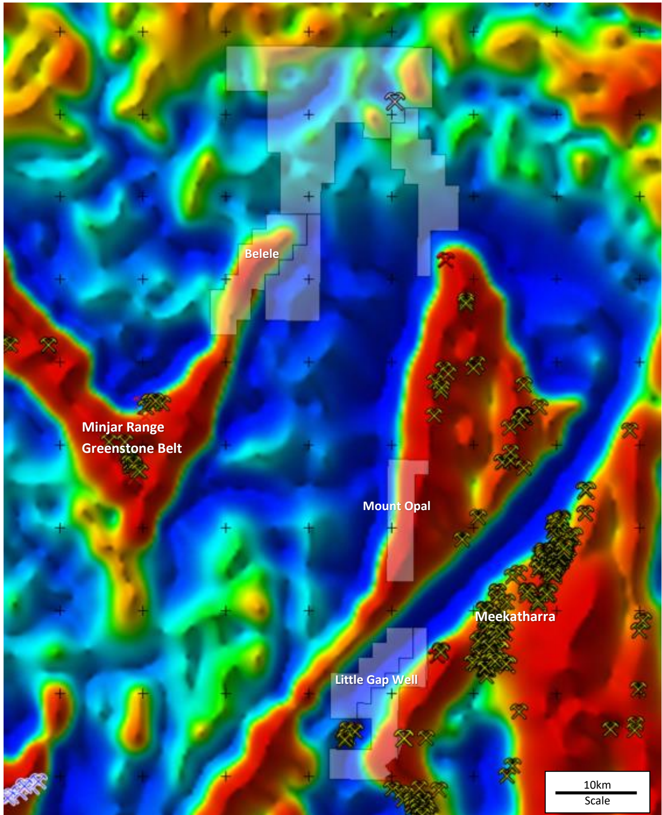
Figure 1. Desert Metals Gold Projects, Meekatharra District. (Background image is Gravity)
