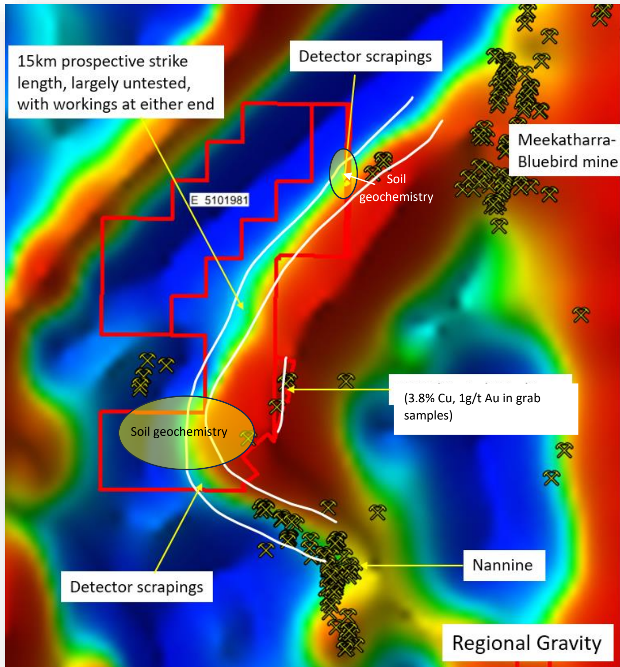
Figure 5 Little Gap Well Project, with approximate areas covered by due diligence soil geochemistry.
