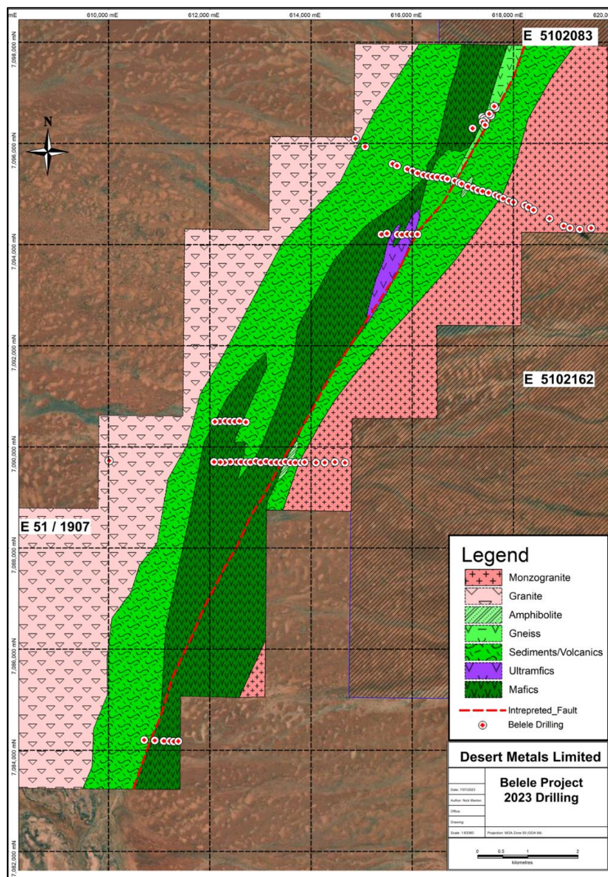
Figure 2 Interpreted Geology based on Drilling within Belele license EL51/1907.
