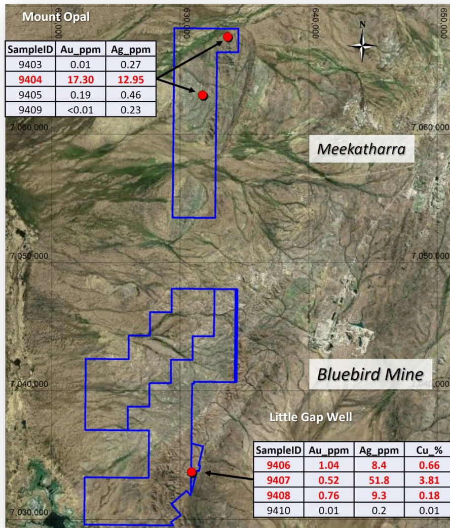
Figure 3. Grab Samples from Little Gap Well and Mount Opal
