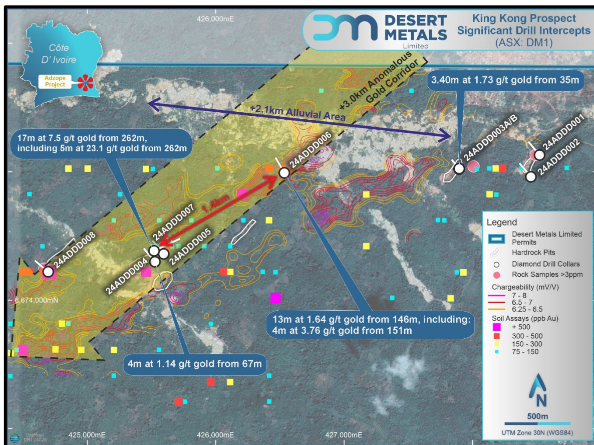
Figure 1 – King Kong Diamond Drilling Plan
