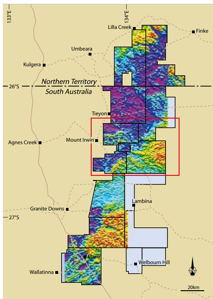
Figure 6 Location of the Abminga Project with airborne EM image.
