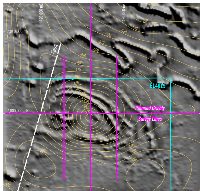
Figure 4 Gravity contours over the magnetic image at Nicholson.
