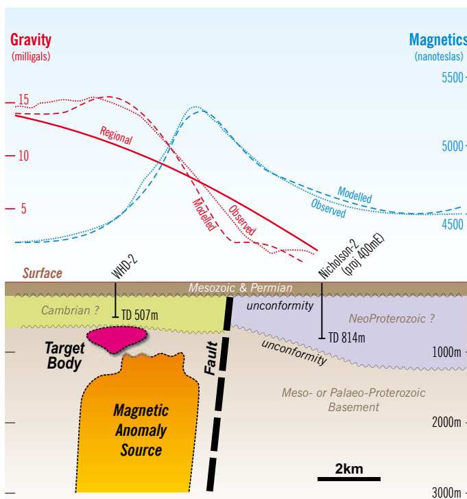
Figure 2 Schematic section of the Welbourn Hill geophysical model.
