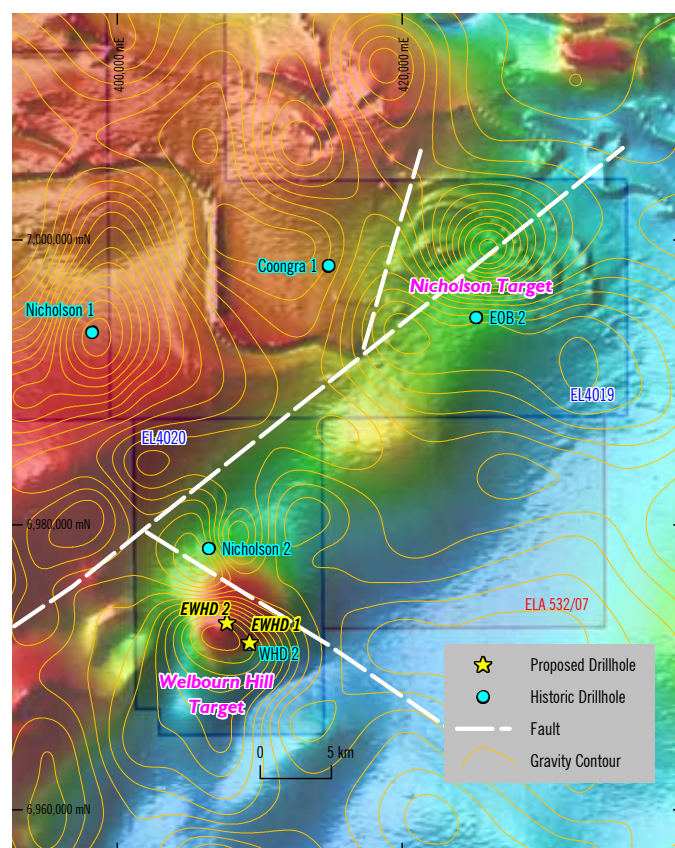
Figure 3 Gravity contours over the magnetic image at Welbourn Hill and Nicholson
