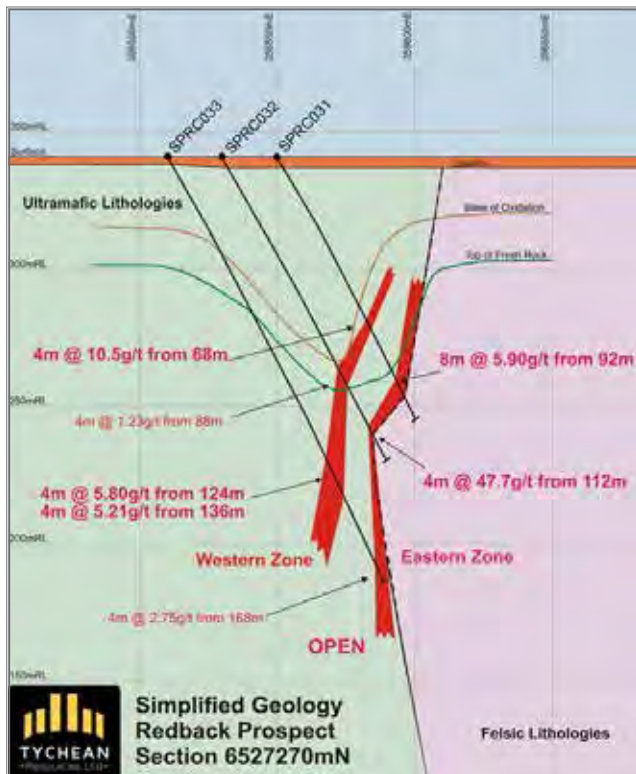
Redback Prospect cross section showing drilling results.
