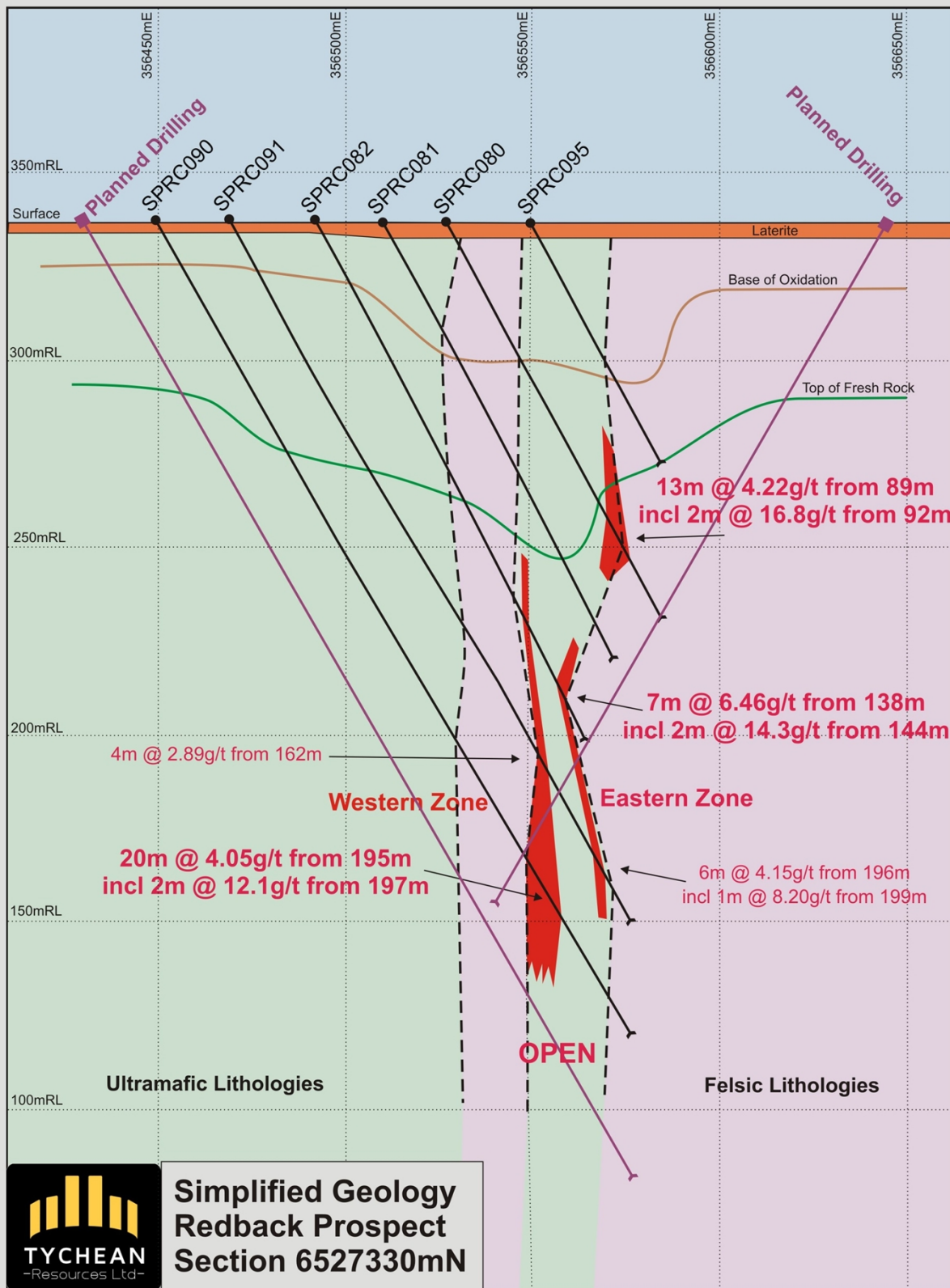
Figure 6 – Redback Prospect – Cross Section 6527330mN \pm 10m
