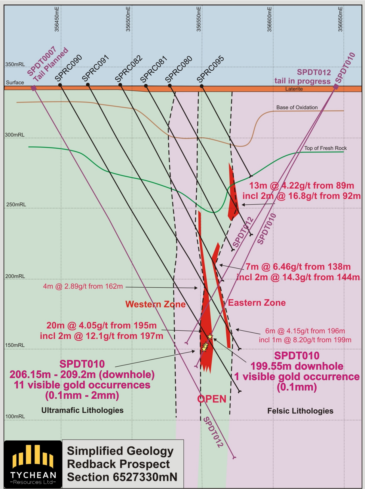
Figure 5 – Redback Prospect – Cross Section 6527330mN \pm 10m
