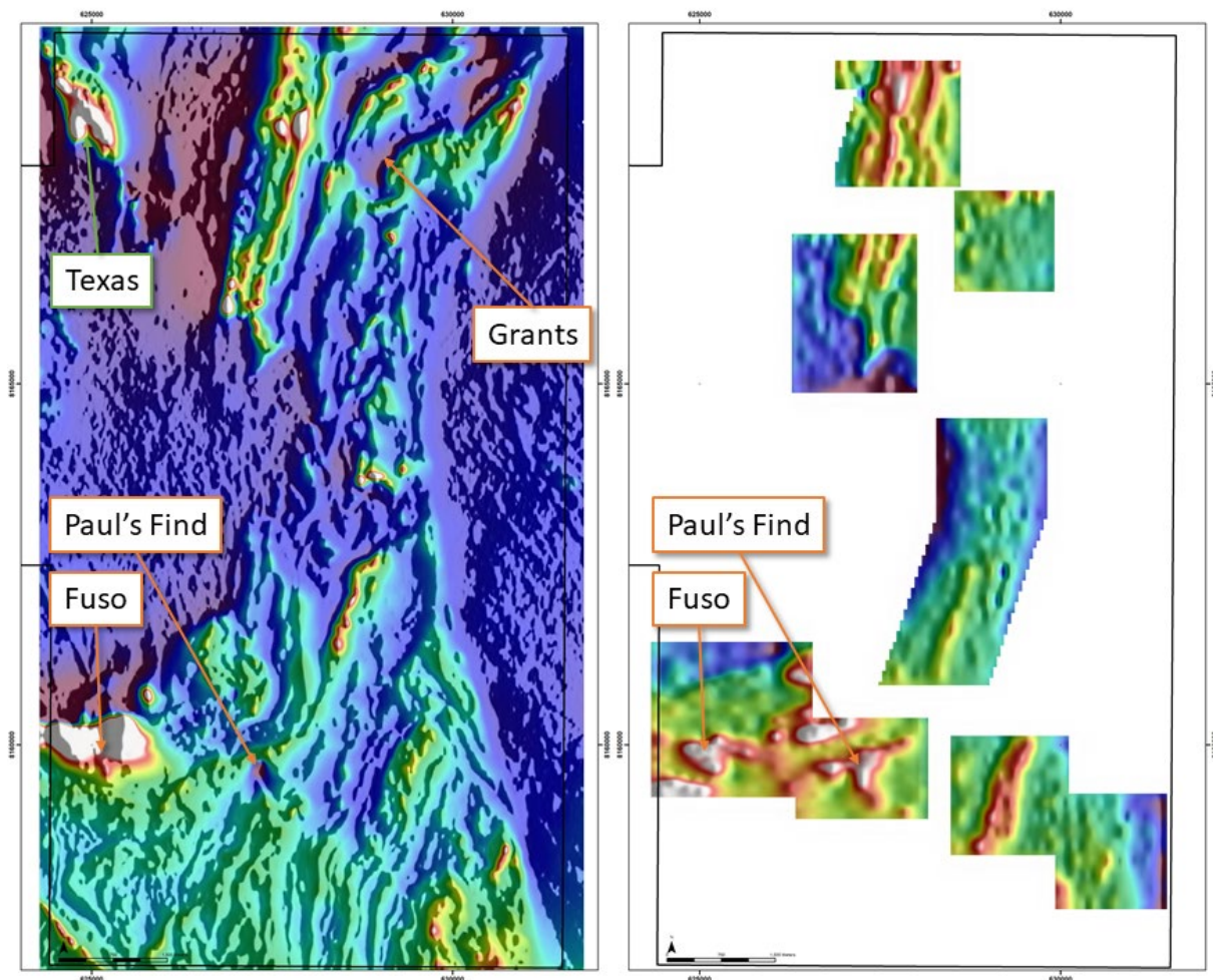
Figure 7: Plan view of the recently acquired airborne magnetics data (L) Reduced to Pole (RTP) and ground gravity (R) Bouguer 1 st vertical derivative highlighting priority target locations.
