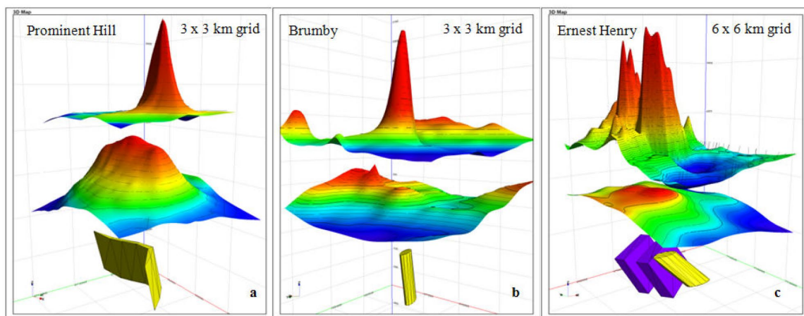
Figure 19: Example of coincident magnetic (top) and gravity (middle) and the resultant inversion modelled bodies (bottom) from Prominent Hill, Brumby and Ernest Henry Proterozoic Cu-Au deposits.
