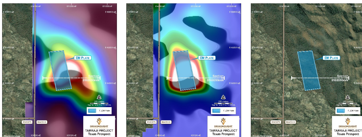
Figure 15: Three images showing the magnetics (L), airborne EM (C), and Ruins Dolerite (R) at Texas.
