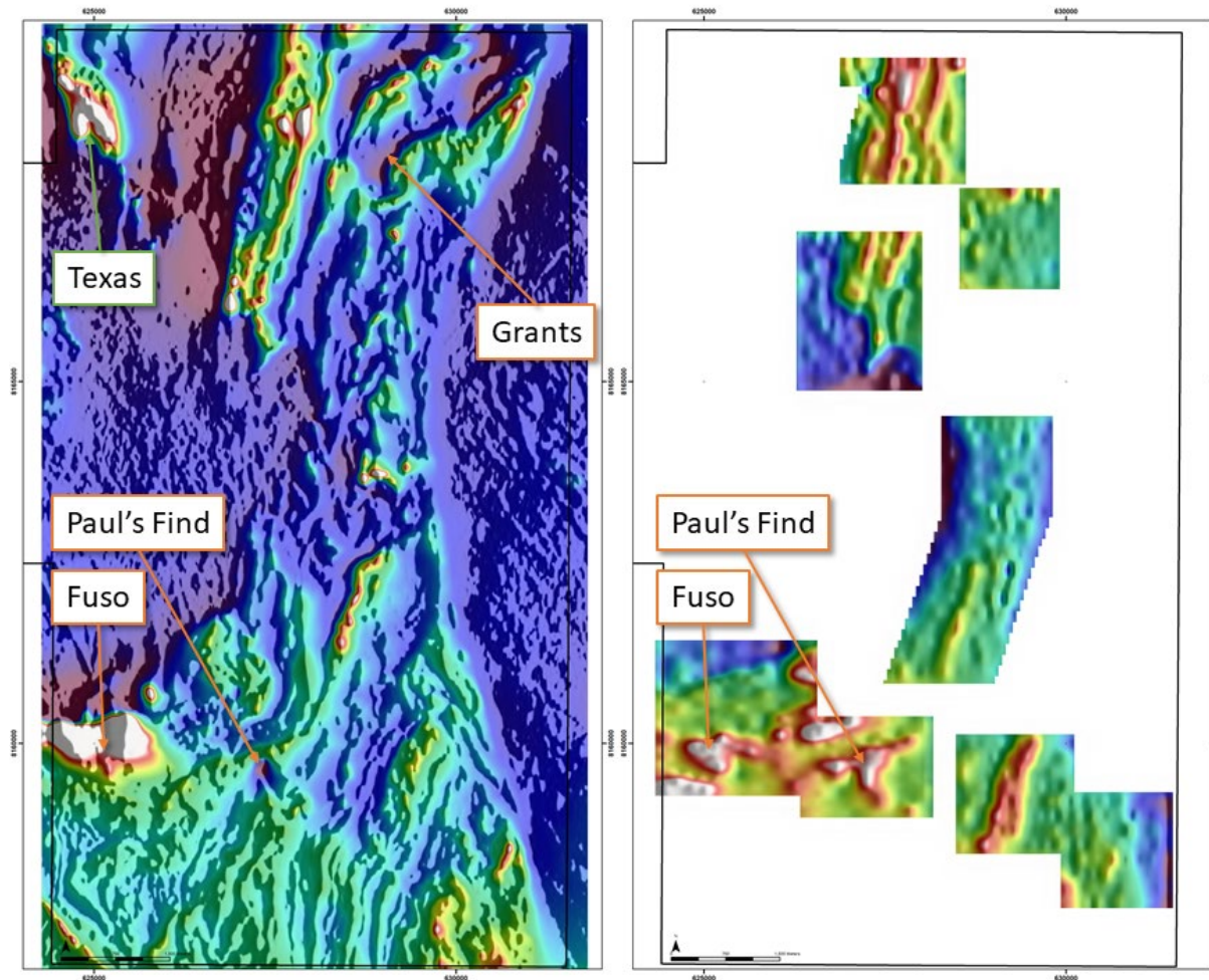
Figure 18: Plan view of the recently acquired airborne magnetics data (L) Reduced to Pole (RTP) and ground gravity (R) Bouguer 1 st vertical derivative highlighting priority target locations.
