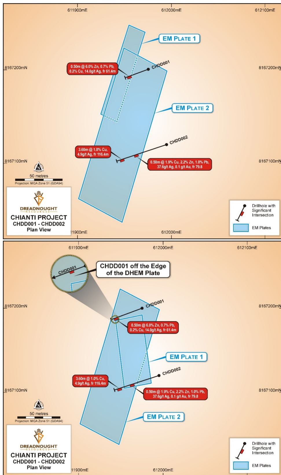
Figure 8: Plan view of the original FLEM plates (top) and remodelled plates (bottom) showing that both holes pierced the original plates as designed (top). However, CHDD001 only clipped the edge of the remodelled upper plate. Further, while CHDD002 intersected both the upper and lower plates, the upper plate sits further south than originally modelled (bottom).
