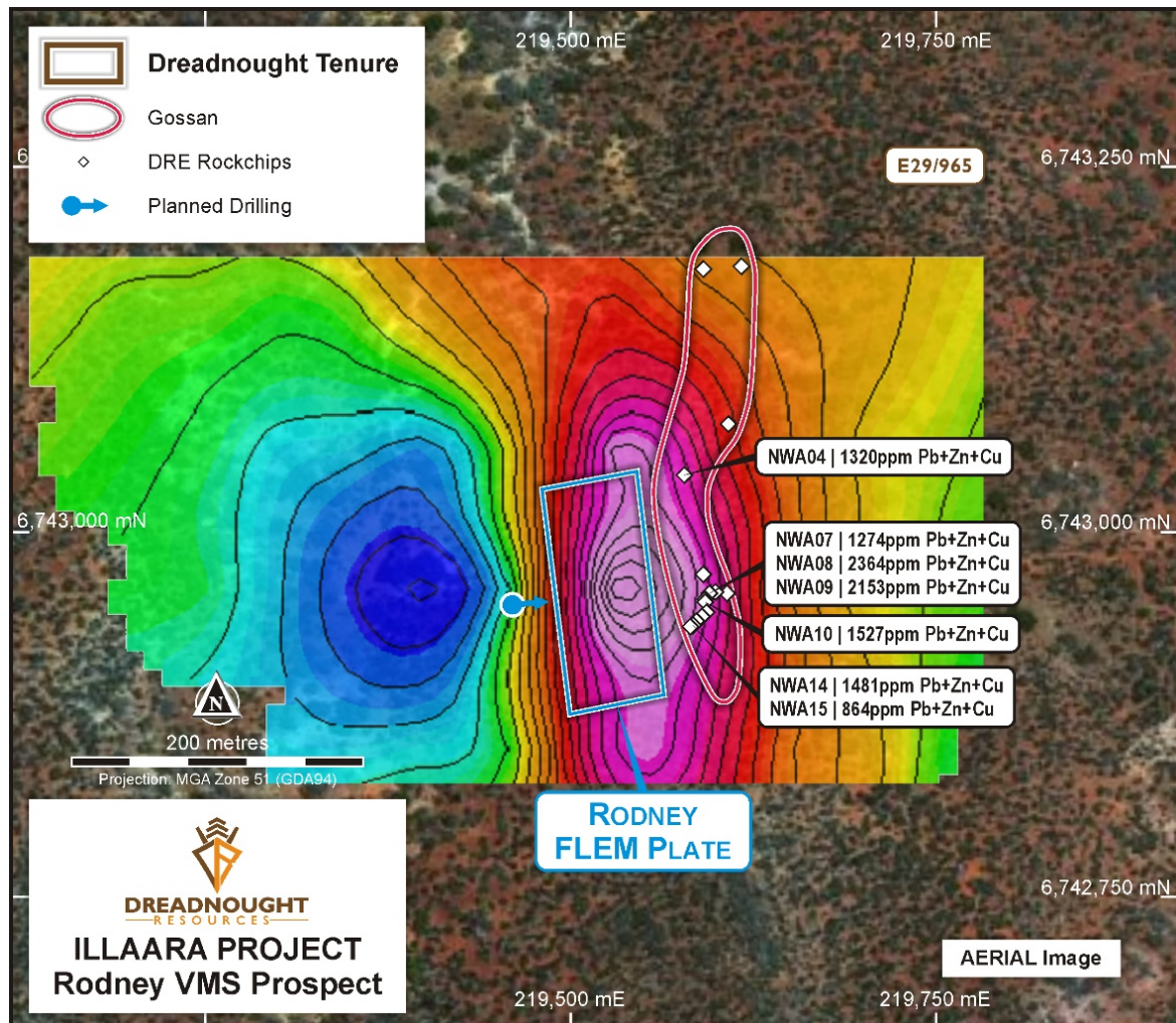
Figure 3: Plan view of Rodney showing the FLEM plate and outcropping gossan over a magnetics image.
