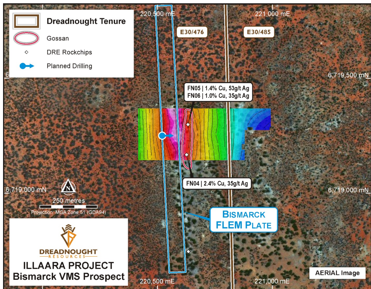
Figure 5: Plan view of Bismarck showing the FLEM plate and outcropping gossan over a late-time conductivity image.
