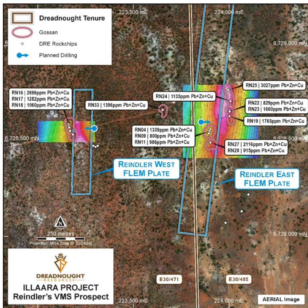
Figure 6: Plan view of Reindler's showing the FLEM plates and outcropping gossans over a late-time conductivity image (Reindler's West) and mid-time conductivity image (Reindler's East).
