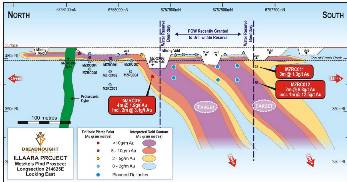
Figure 3: Long section of Metzke's Find showing the extent of historic workings and follow up drill targets beneath the deeper workings.
