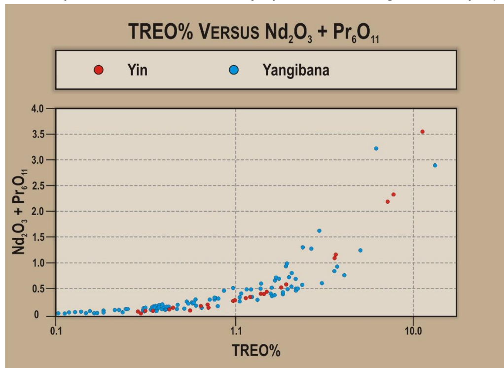
Figure 9: Scatter plot showing the similarity of TREO and Nd_2O_3 + Pr_6O_{11} values from Yin and publicly available Yangibana rock chip data.
