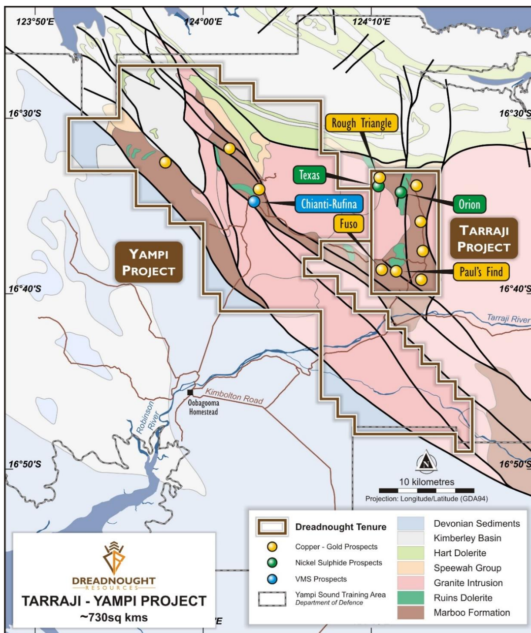
Figure 2: Plan view of Tarraji-Yampi showing targets over solid geology.
