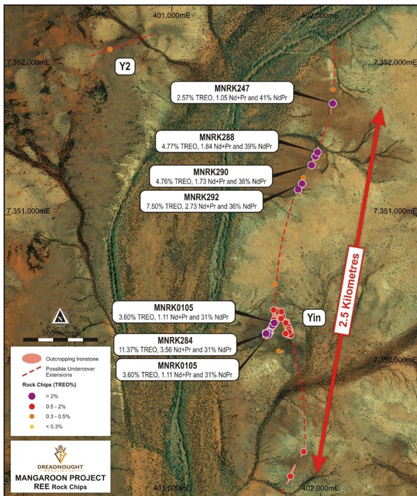
Figure 7: Map showing the location of rock chip samples at Yin and the location of ~2.5kms of outcropping ironstones and their interpreted extensions under shallow cover.
