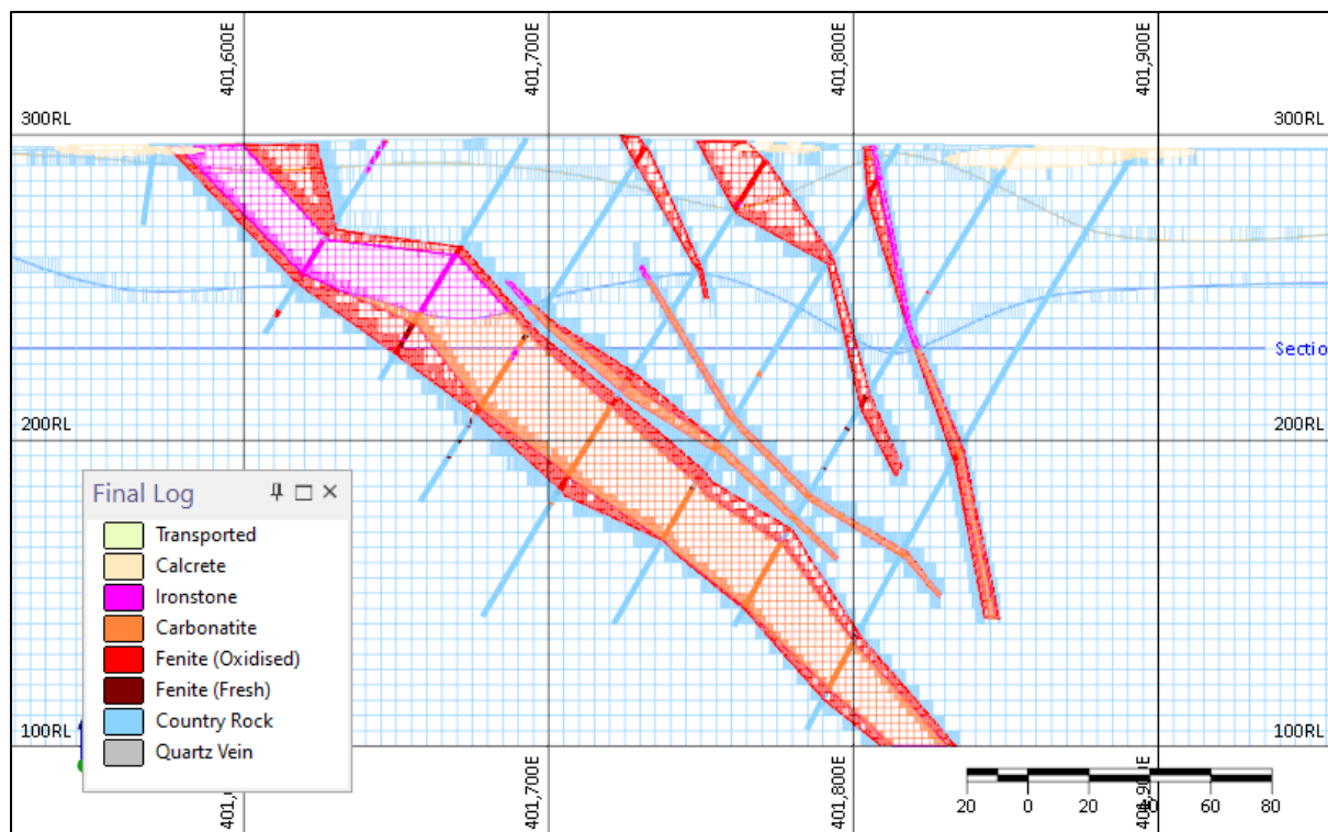
Figure 6: Rock model lithology highlighting ironstone, carbonatite and fenite
